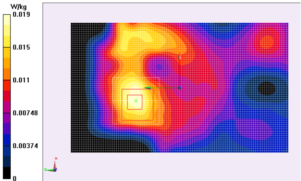
Fig.10 2450 MHz CH11
