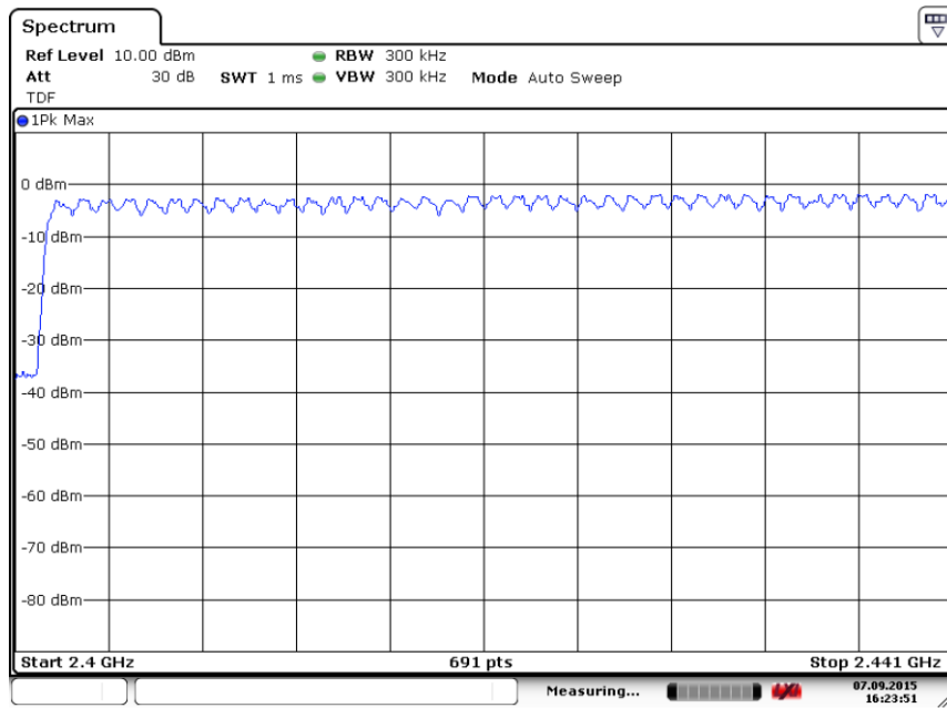
Fig. 89 Hopping channel ch0~39 ( \pi/4 DQPSK, Ch39)
