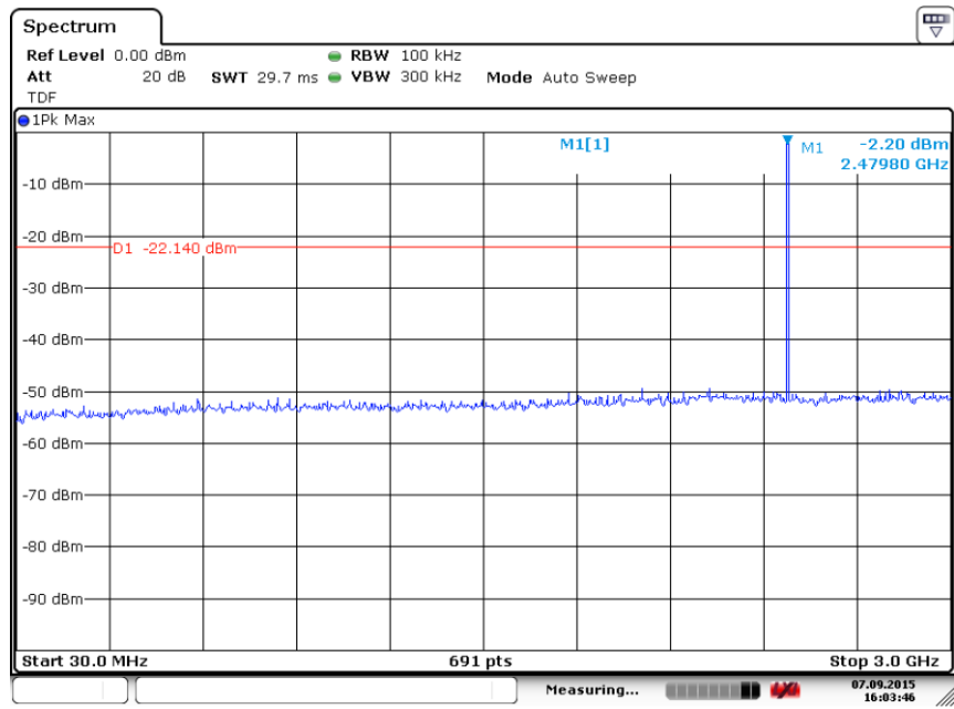
Fig. 47 Conducted Spurious Emission (8DPSK, Ch78, 30 MHz-3 GHz)
