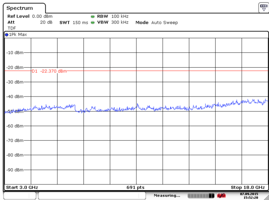
Fig. 30 Conducted Spurious Emission (GFSK, Ch78, 3GHz-18 GHz)
