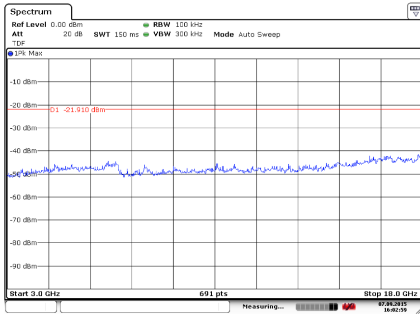
Fig. 45 Conducted Spurious Emission (8DPSK, Ch39, 3GHz-18 GHz)
