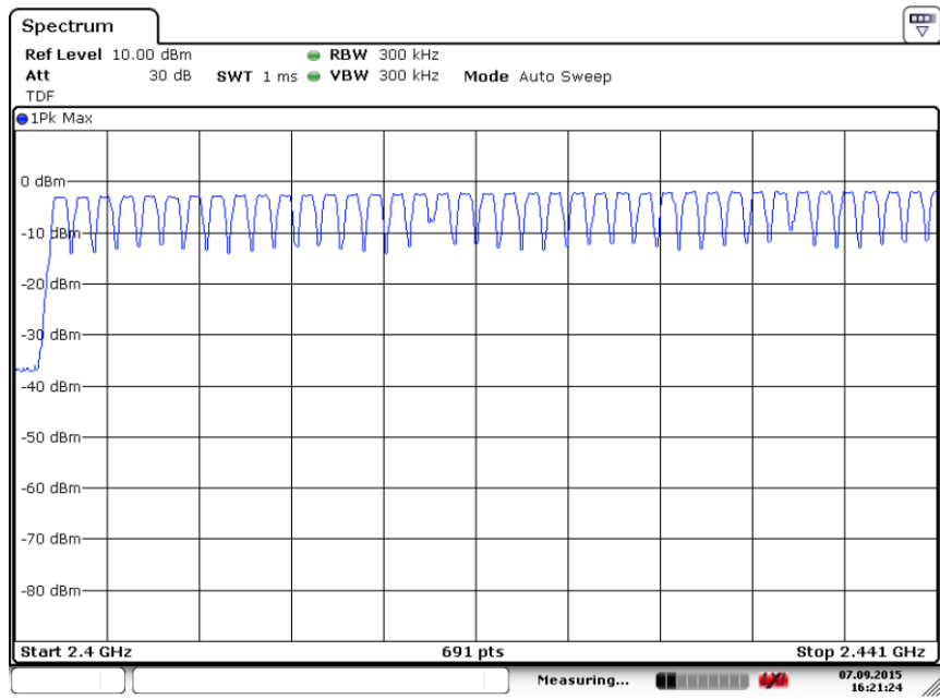
Fig. 87 Hopping channel ch0~39 (GFSK, Ch39)
