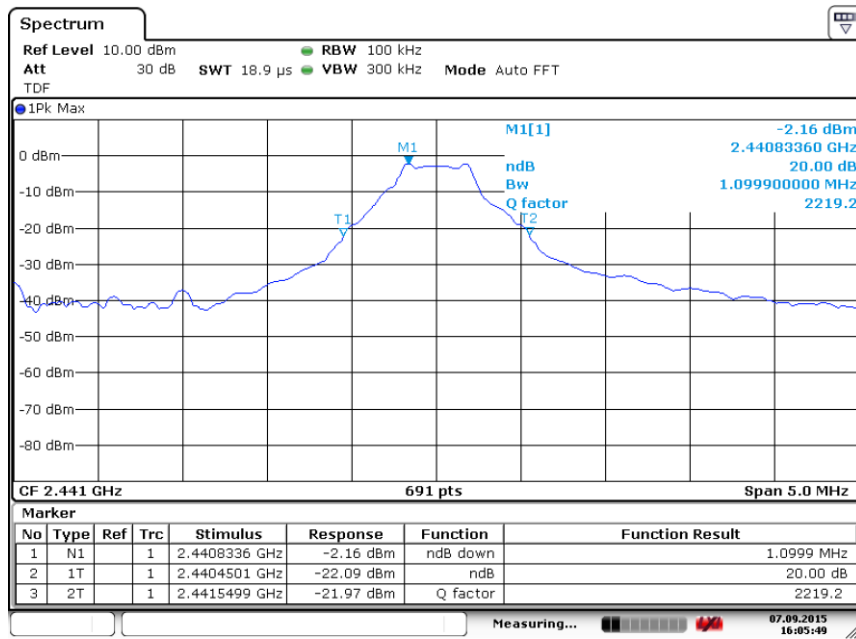
Fig. 73 Occupied 20dB Bandwidth (GFSK, Ch 39)
