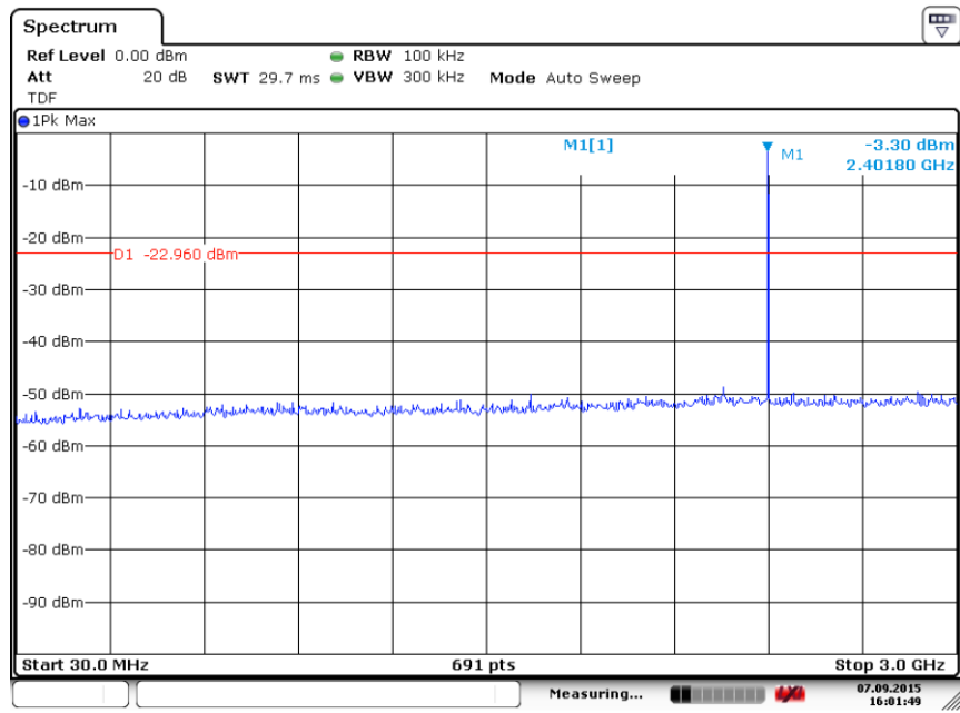
Fig. 41 Conducted Spurious Emission (8DPSK, Ch0, 30 MHz-3 GHz)
