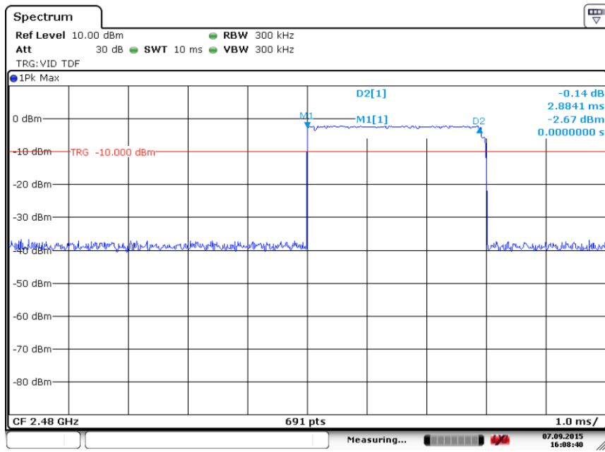
Fig. 81 Time of Occupancy(Dwell Time) (GFSK, Ch39)
