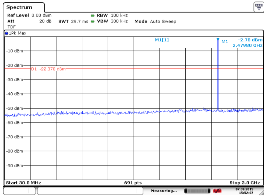
Fig. 29 Conducted Spurious Emission (GFSK, Ch78, 30 MHz-3 GHz)
