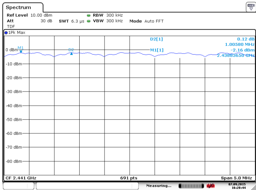
Fig. 93 Carrier Frequency Separation (GFSK, Ch39)
