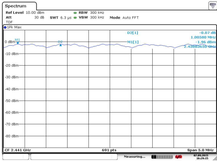
Fig. 95 Carrier Frequency Separation (8DPSK, Ch39)
