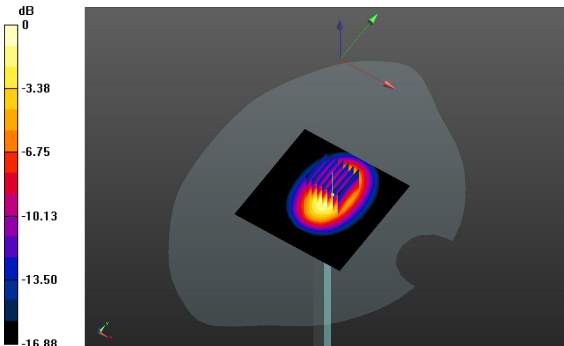
0 dB = 3.97 W/kg
