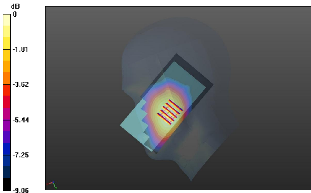
0 dB = 0.164 W/kg
