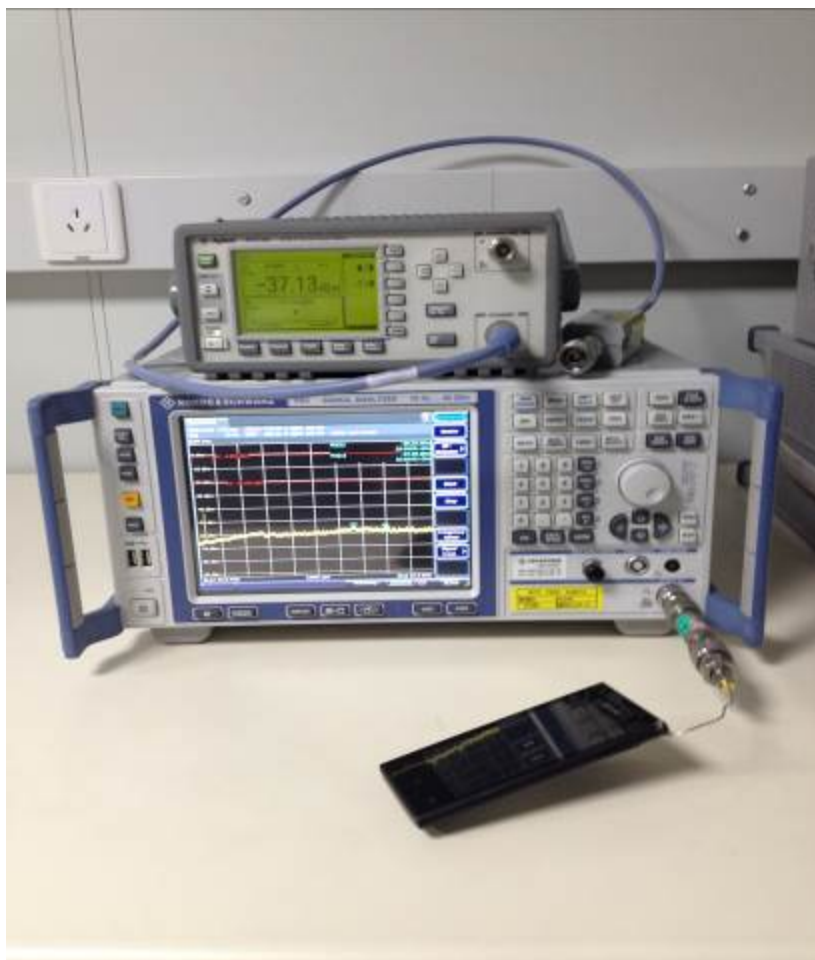
Spurious RF Conducted Emissions Test setup
