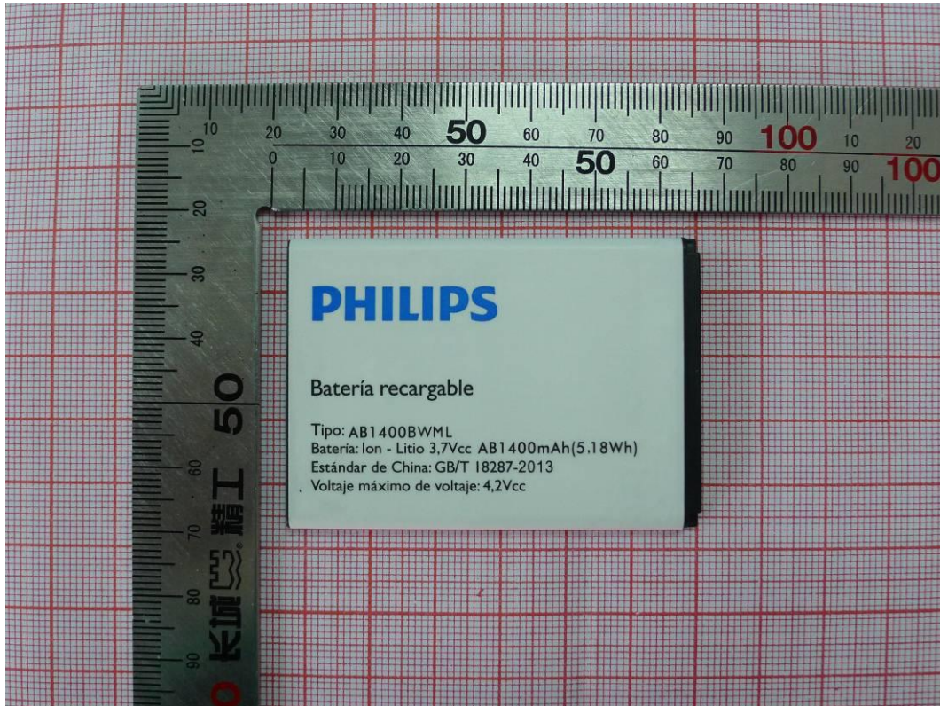
Battery AB1400BWML
