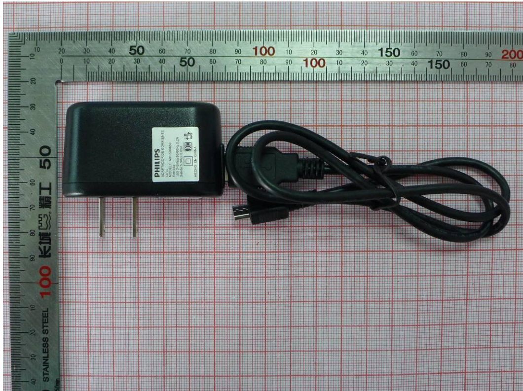
Charger A31-500650
