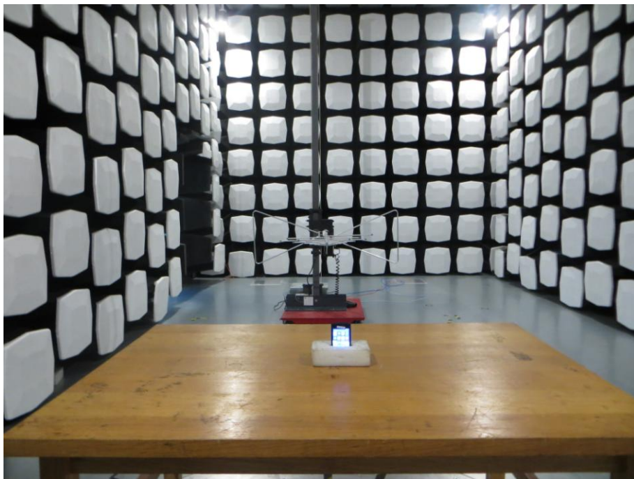
6. Radiated Emissions (Part 15C) (Above 1GHz)
