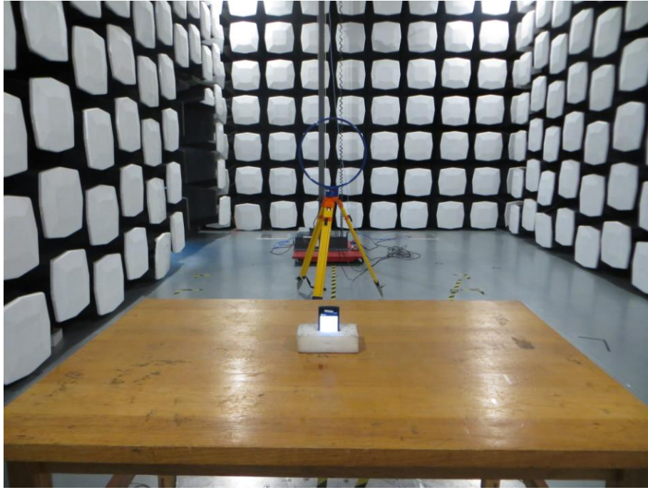
5. Radiated Emissions (Part 15C) (below 1GHz)
