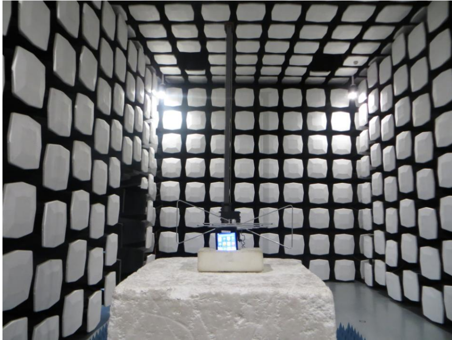
7. Radiated Emissions (Part 22/24) (below 3GHz)
