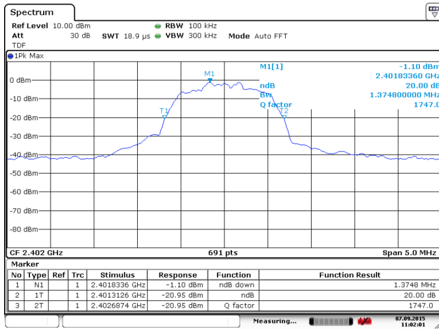
Fig. 75 Occupied 20dB Bandwidth ( \pi/4 DQPSK, Ch 0)
