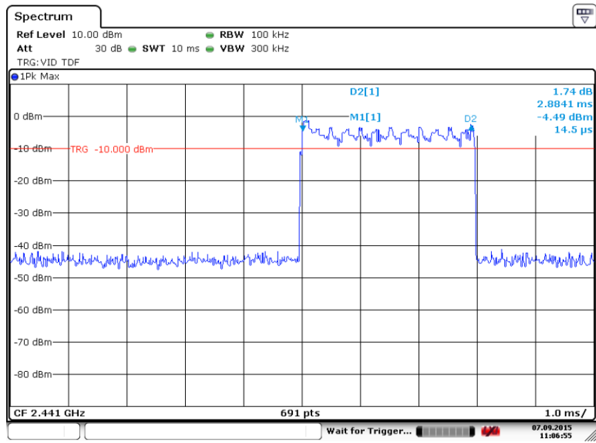
Fig. 83 Time of Occupancy(Dwell Time) ( \pi/4 DQPSK, Ch39)
