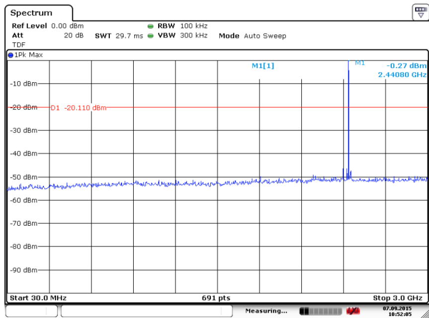
Fig. 26 Conducted Spurious Emission (GFSK, Ch39, 30 MHz-3 GHz)
