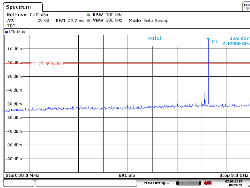
Fig. 47 Conducted Spurious Emission (8DPSK, Ch78, 30 MHz-3 GHz)
