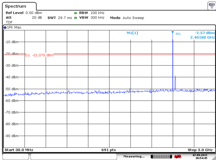
Fig. 31 Conducted Spurious Emission ( \pi/4 DQPSK, Ch0, 2.402GHz)
