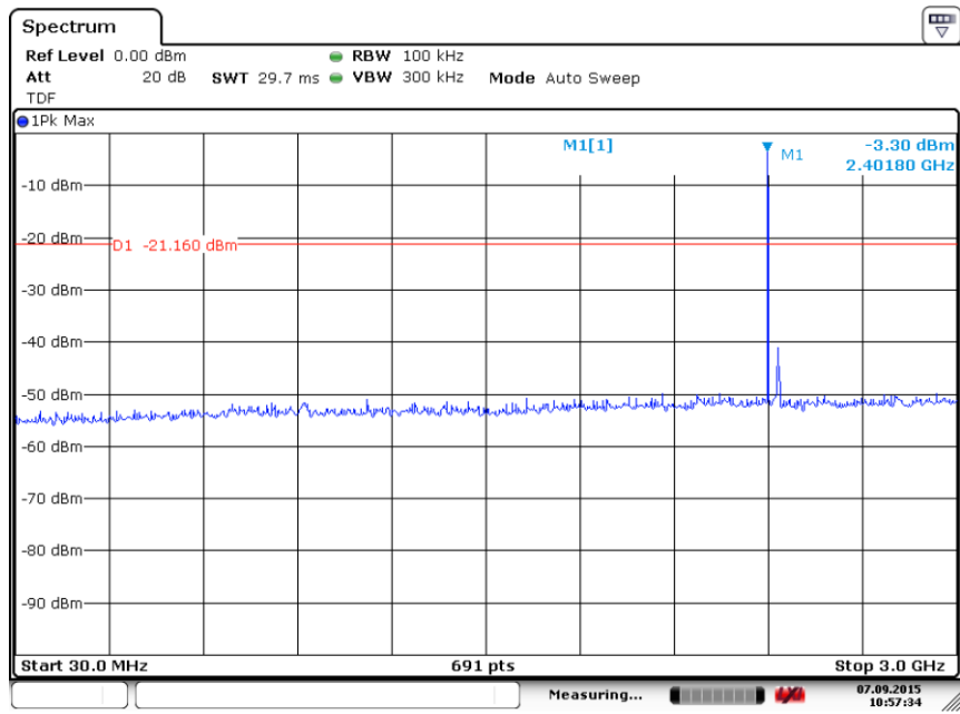
Fig. 41 Conducted Spurious Emission (8DPSK, Ch0, 30 MHz-3 GHz)
