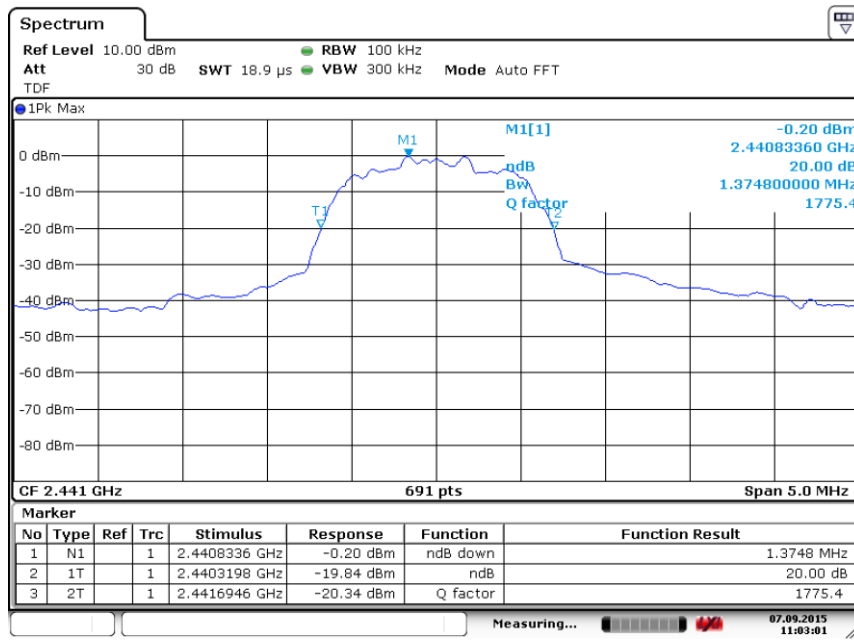
Fig. 79 Occupied 20dB Bandwidth (8DPSK, Ch 39)
