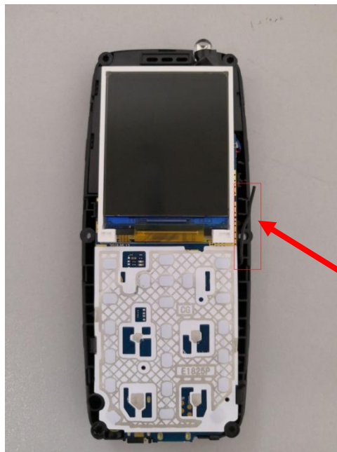
BT Antenna
