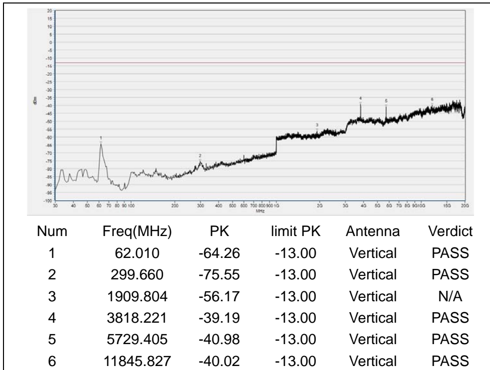
(Plot D6, GPRS 1900MHz, Channel = 810, Vertical)
