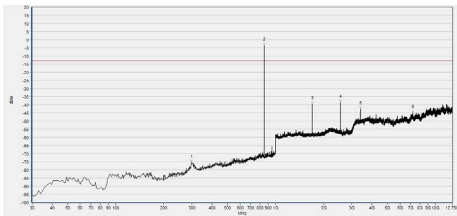
(Plot C4, GPRS 850MHz, Channel = 190, Vertical)
