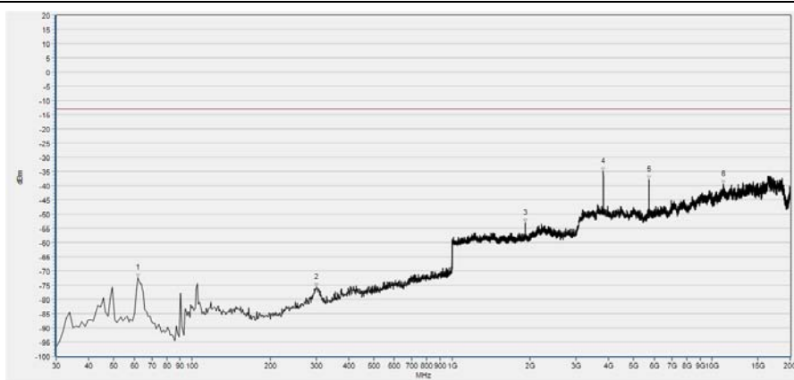
(Plot B4, GSM 1900MHz, Channel = 661, Vertical)
