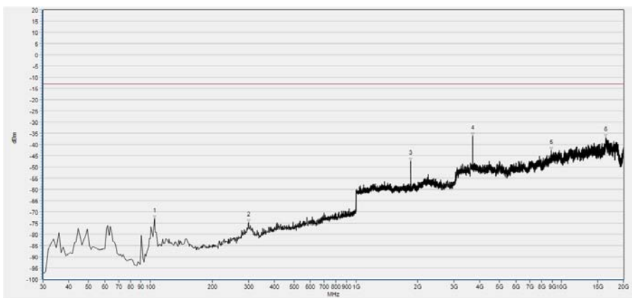
(Plot C6, GPRS 850MHz, Channel = 251, Vertical)
