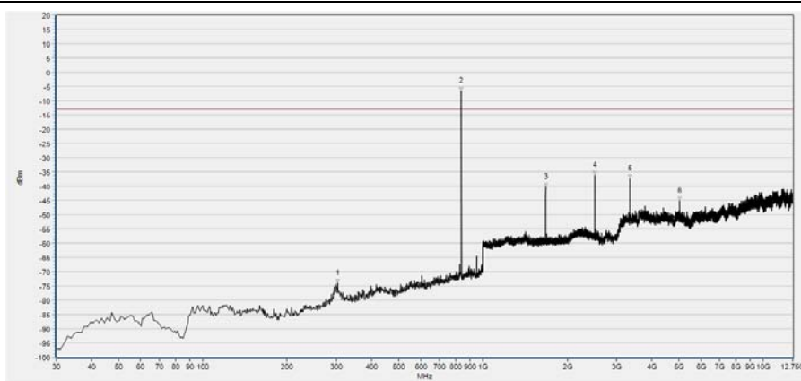
(Plot C2, GPRS 850MHz, Channel = 128, Vertical)
