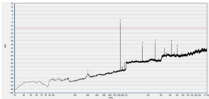
(Plot A2, GSM 850MHz, Channel = 128, Vertical)
