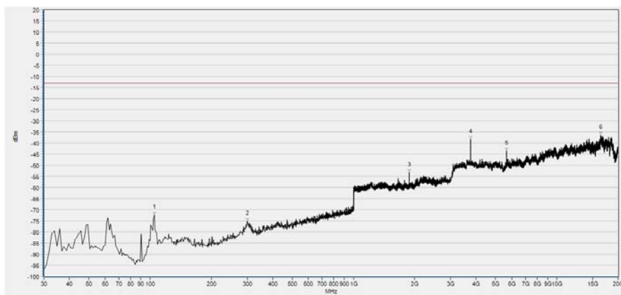
(Plot D2, GPRS 1900MHz, Channel = 512, Vertical)
