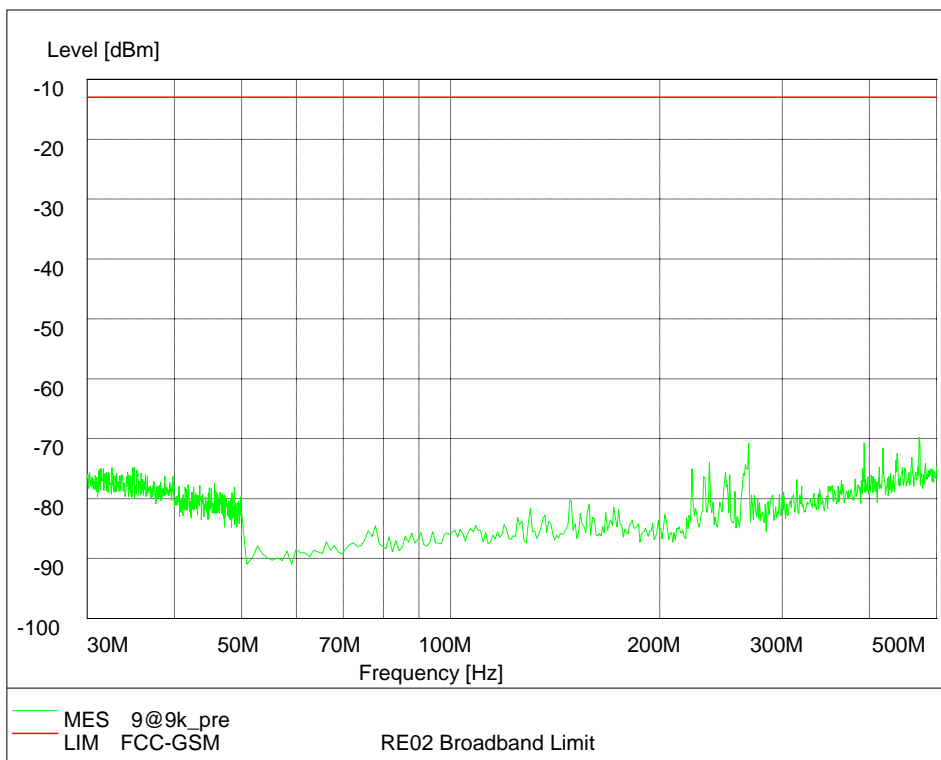
Channel 661, 30MHz~500MHz (Traffic Mode)
