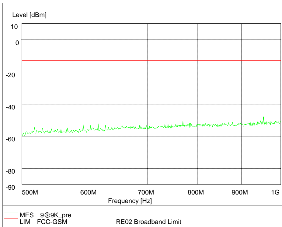
Channel 661, 500MHz~1GHz (Traffic Mode)
