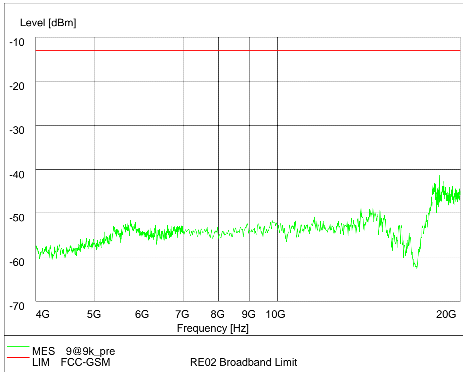
Channel 661, 4GHz~20GHz(Traffic Mode)
