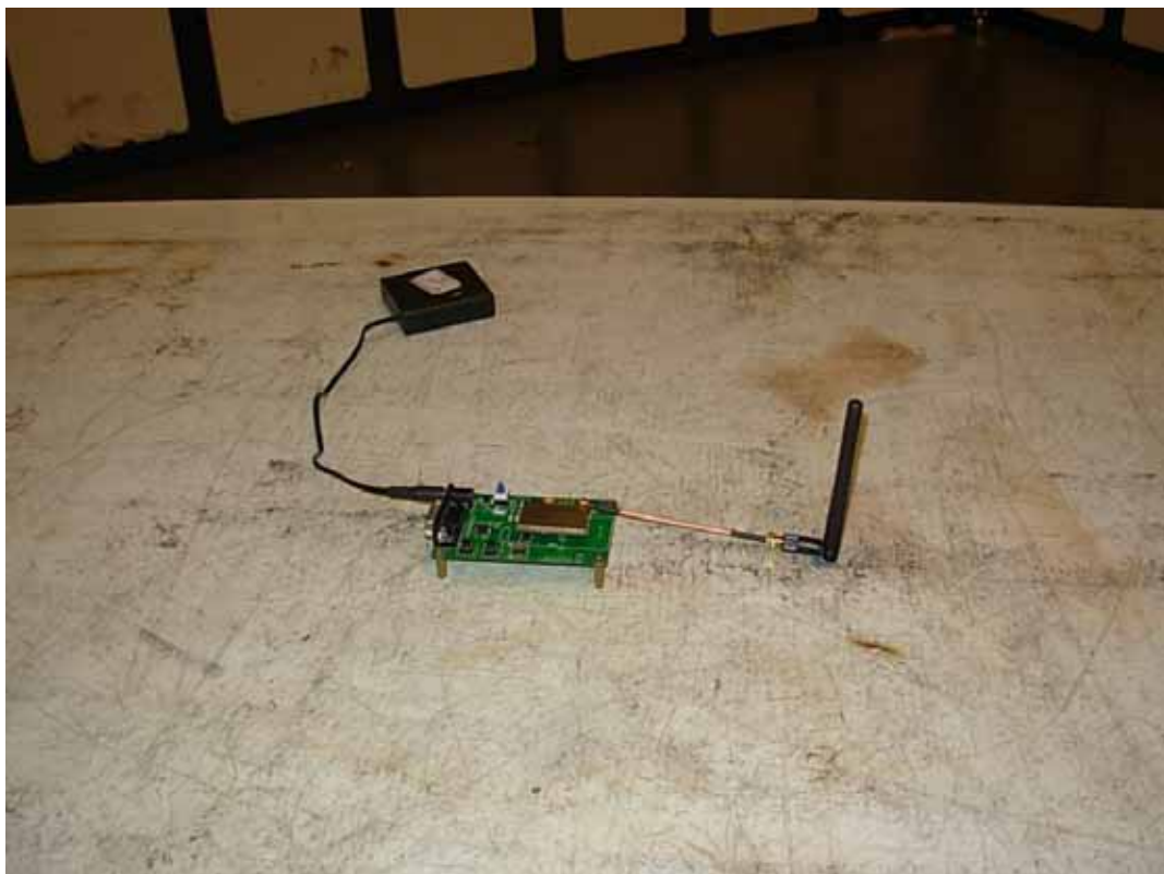
ZOOM VIEW OF RADIATED EMISSION TEST (ANTENNA 2)
