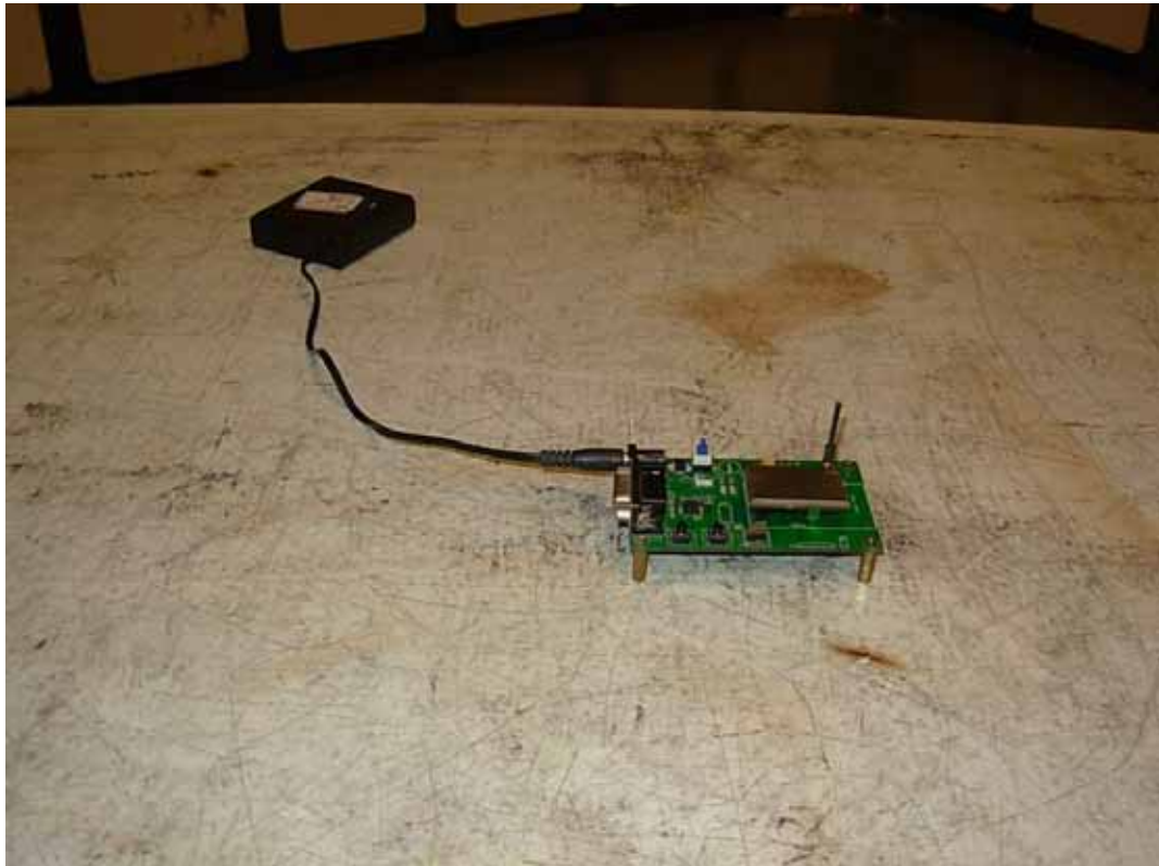
ZOOM VIEW OF RADIATED EMISSION TEST (ANTENNA 1)
