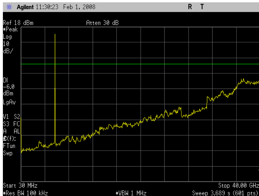
802.11/a – Mid Channel Conducted Emissions 30MHz – 40GHz
