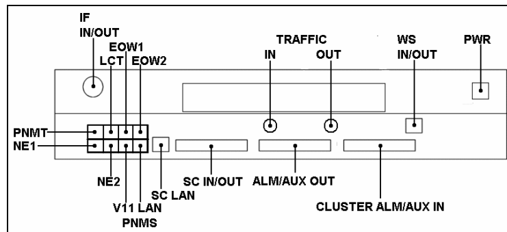
Figure 2. Block Diagram of Ports Identification
