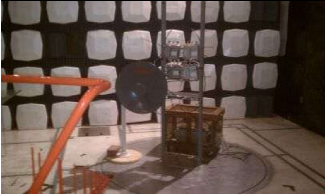
Photograph 1. Radiated Emissions, Test Setup, LF
