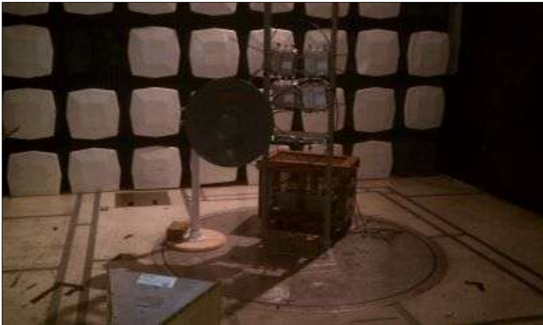
Photograph 4. Radiated Spurious Emissions, Test Setup, HF
