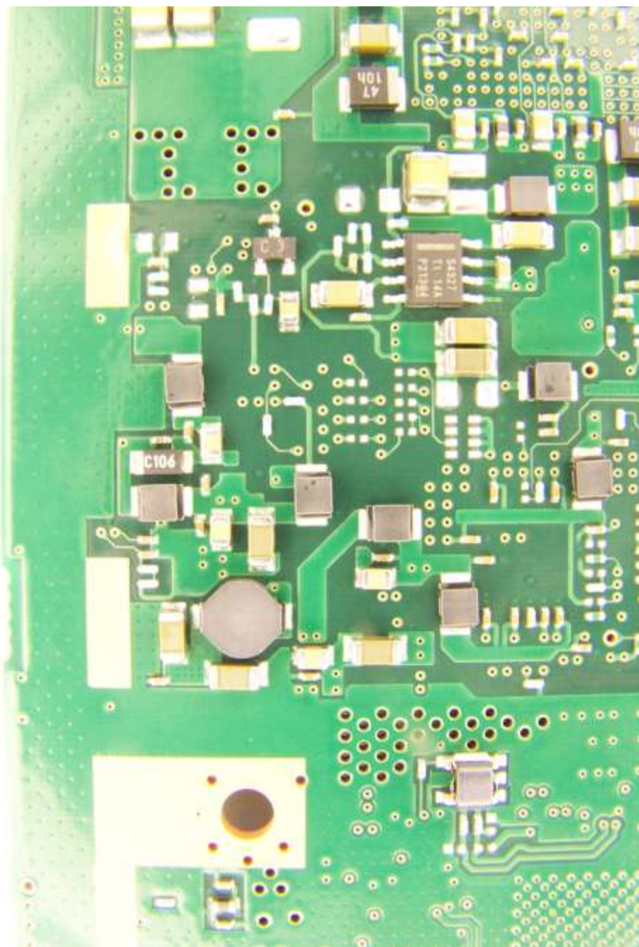
Photograph 30. Modem Components 10
