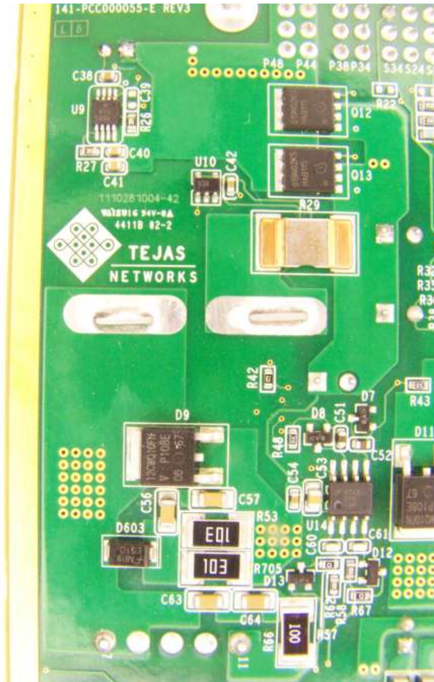
Photograph 37. PS components 3
