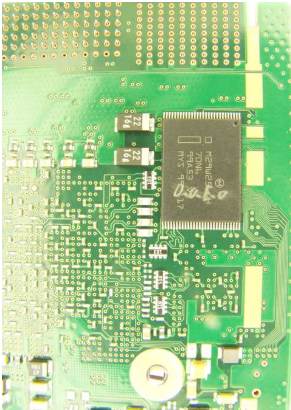
Photograph 28. Modem Components 8
