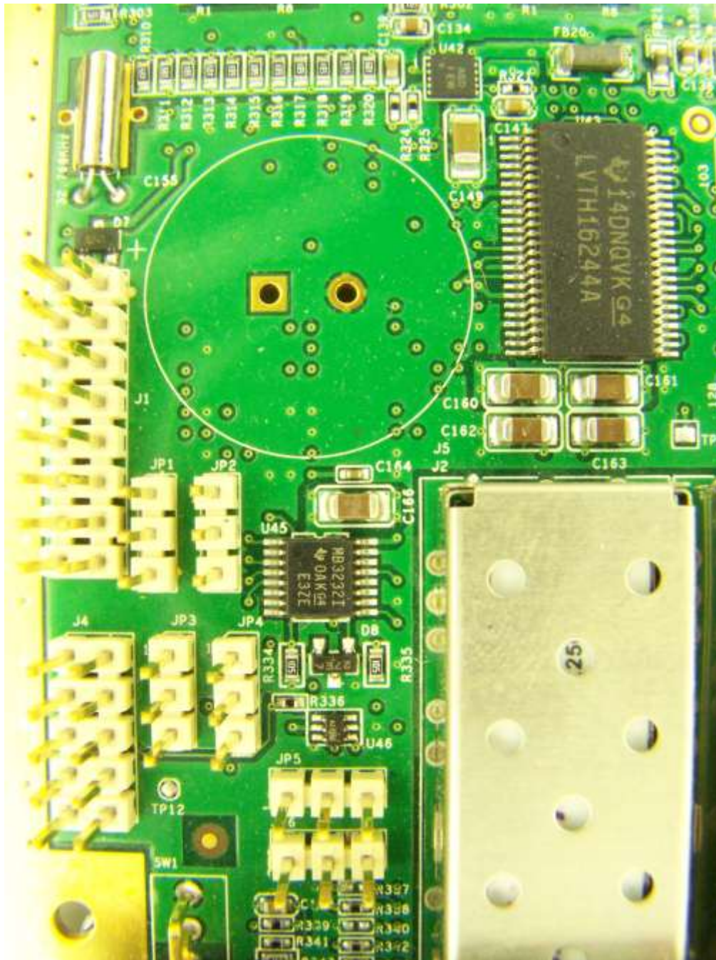
Photograph 9. Interface board components 7
