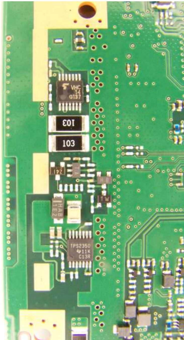
Photograph 31. Modem Components 11
