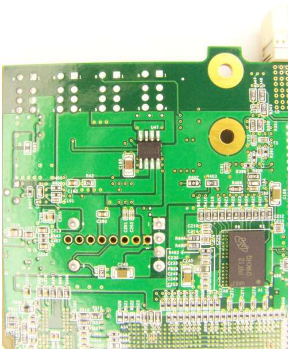
Photograph 14. Interface board components 12
