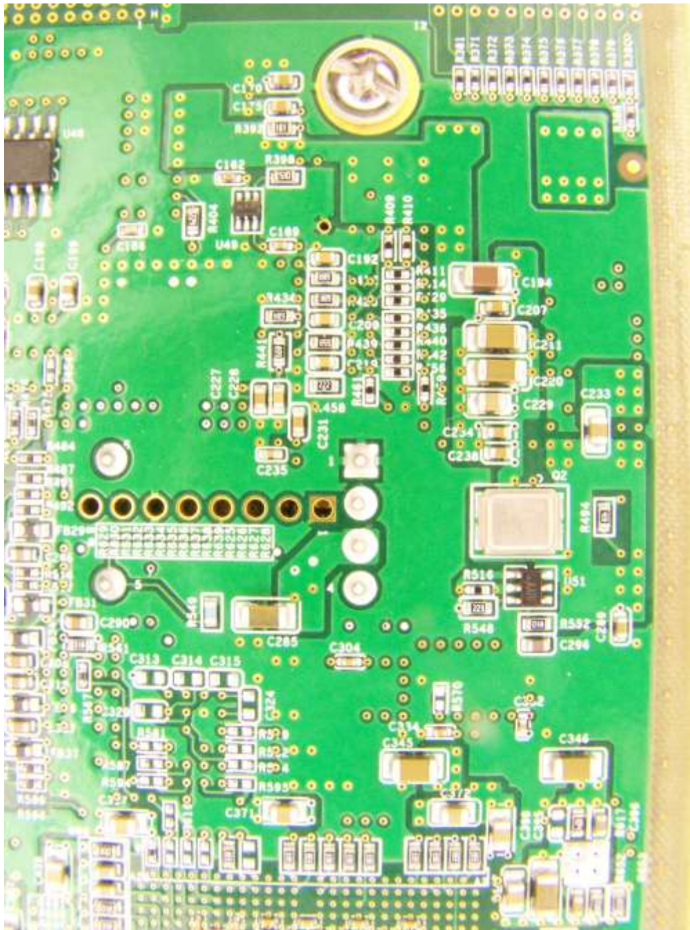
Photograph 16. Interface board components 14
