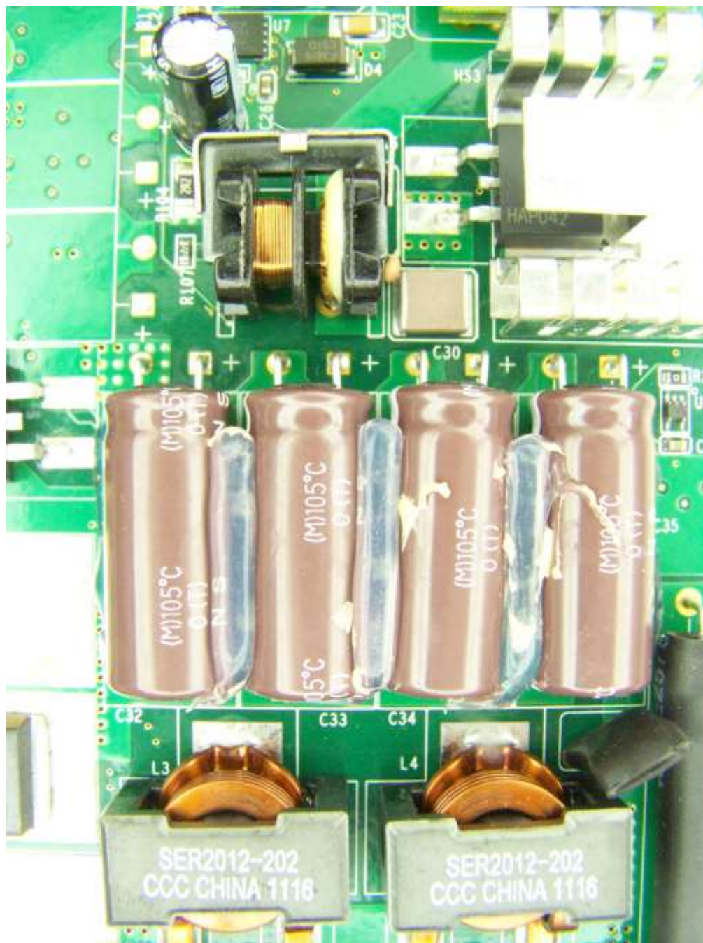
Photograph 45. PS components 11
