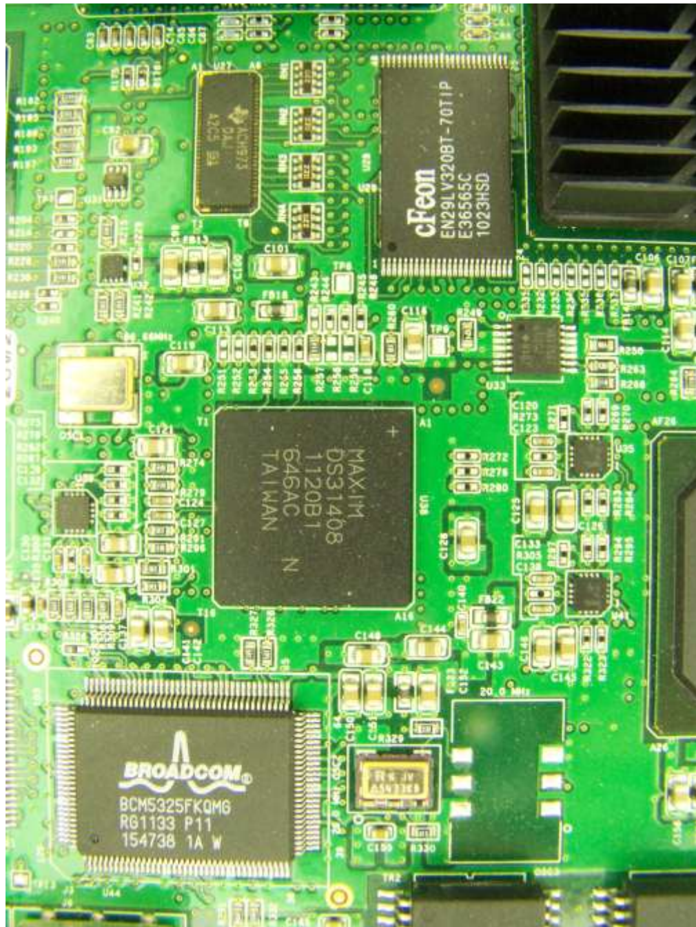
Photograph 7. Interface board components 5
