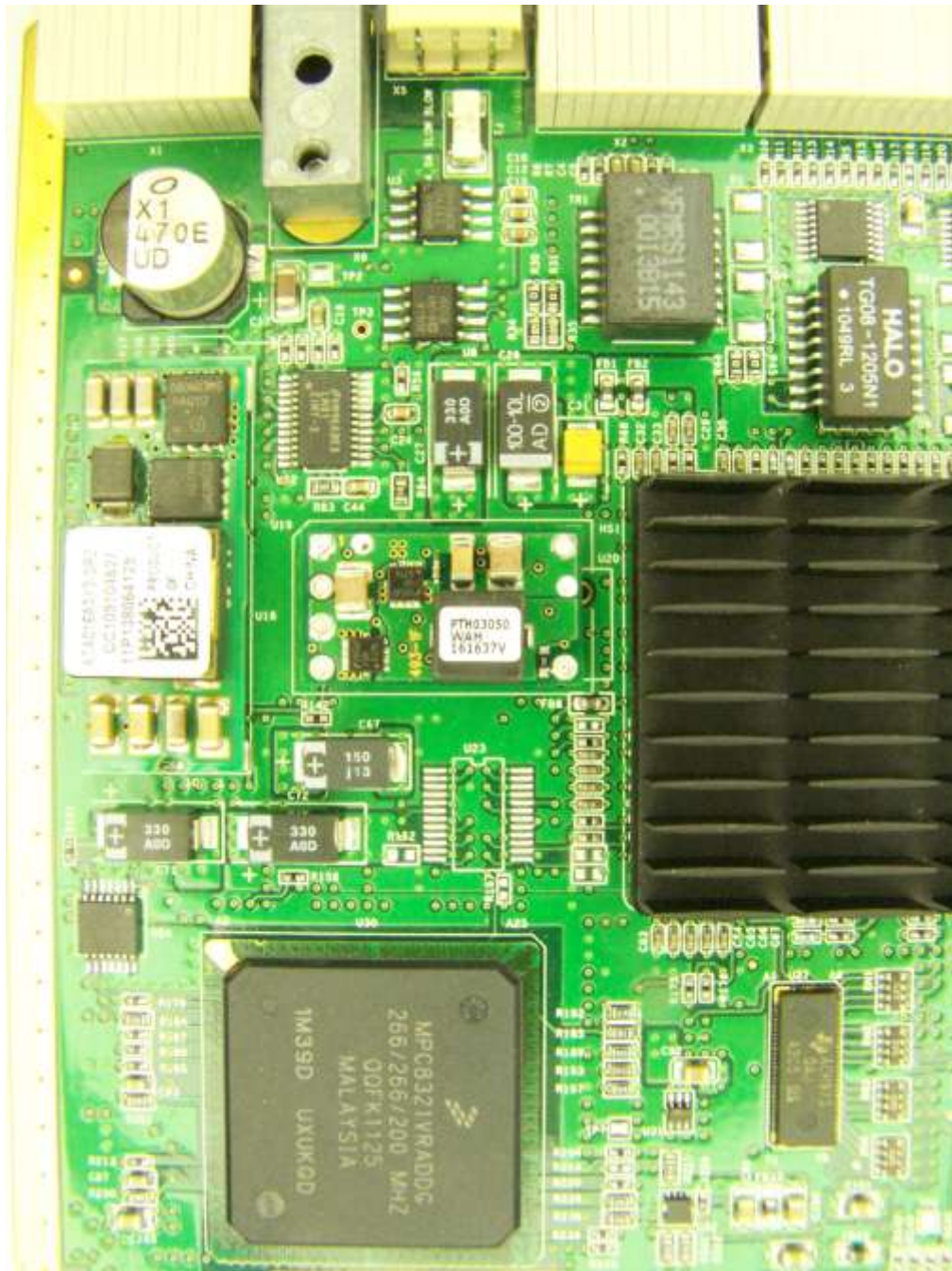
Photograph 3. Interface board components 1
