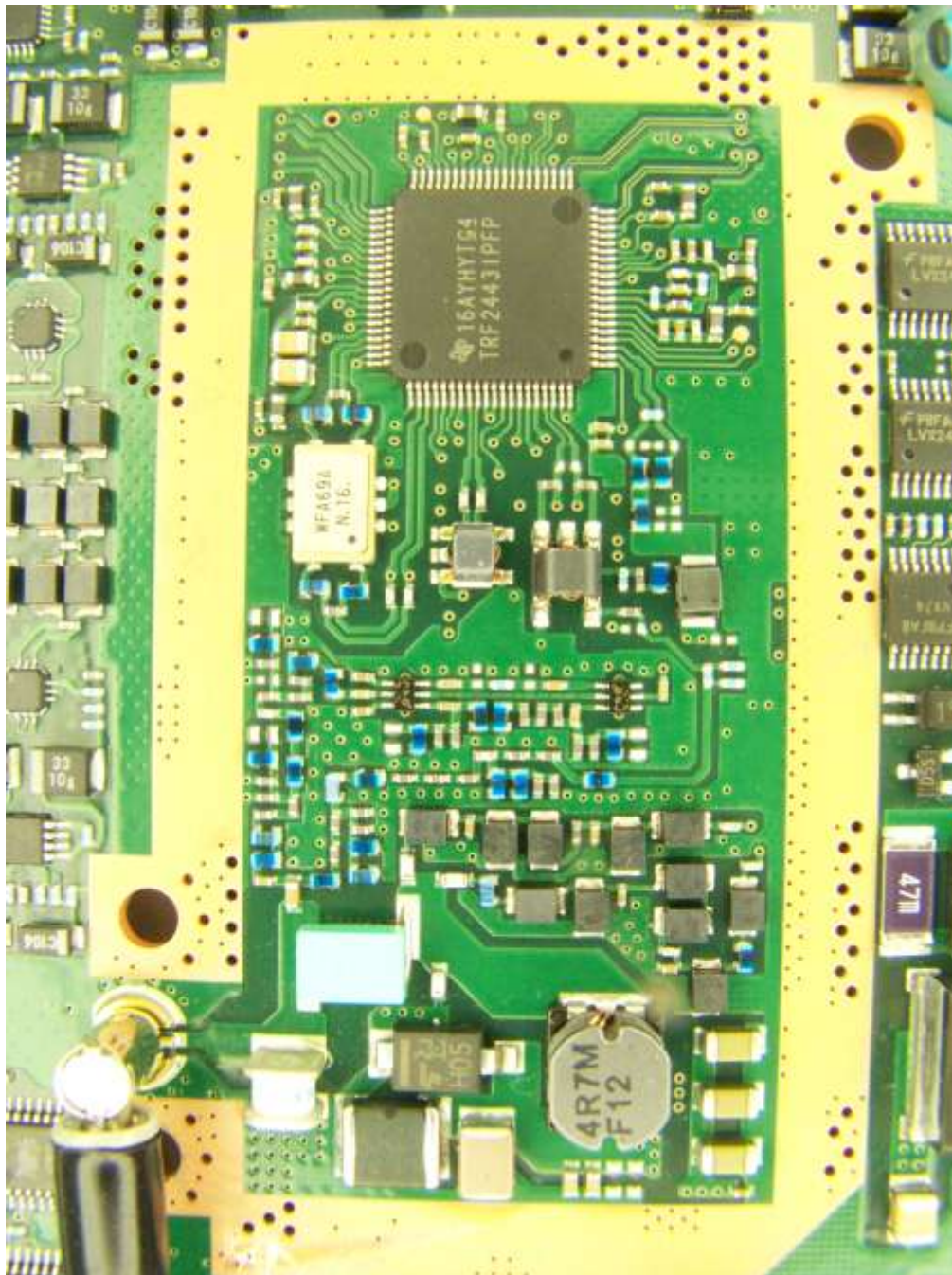
Photograph 20. Modem under shield
