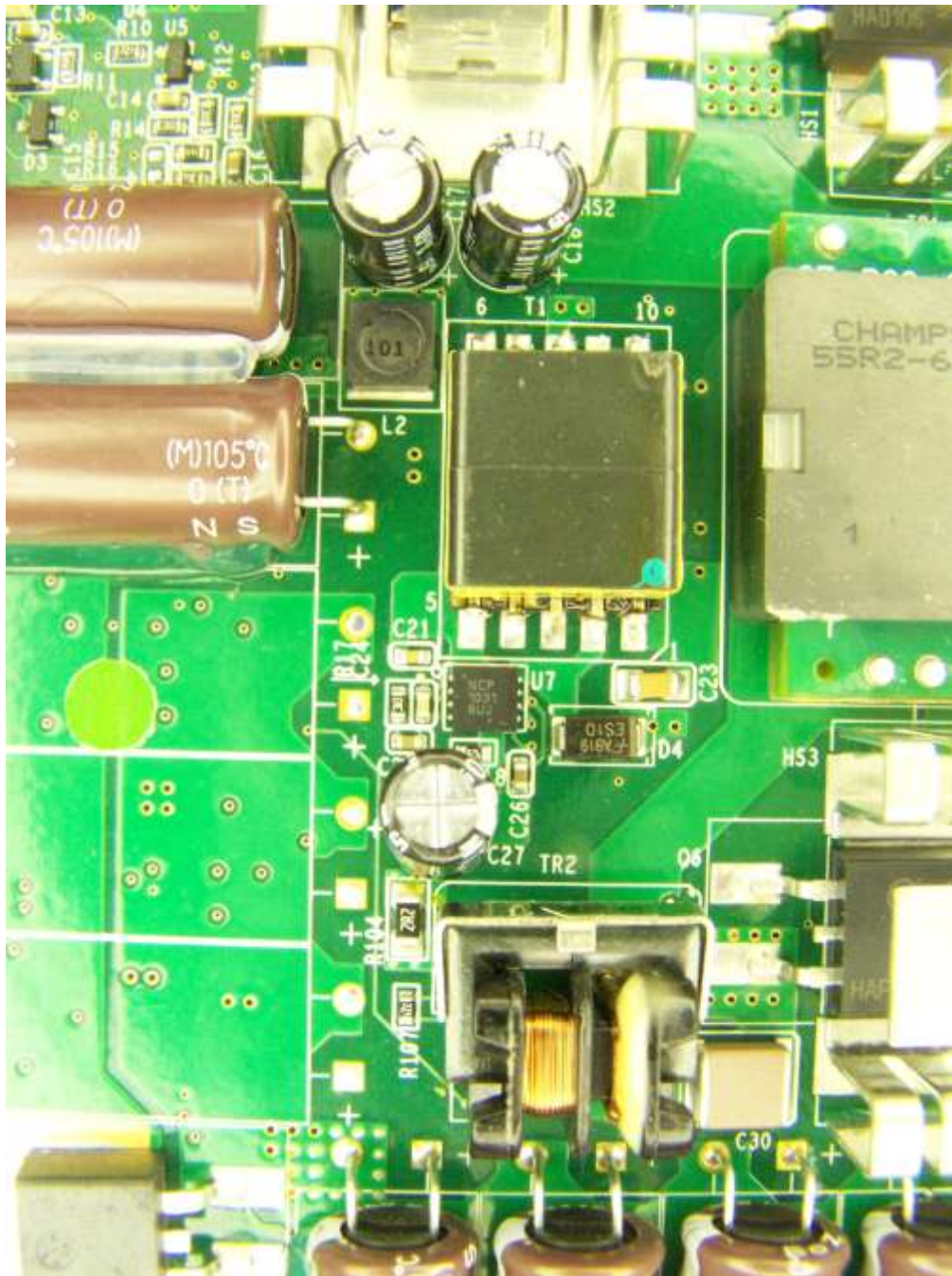
Photograph 44. PS components 10
