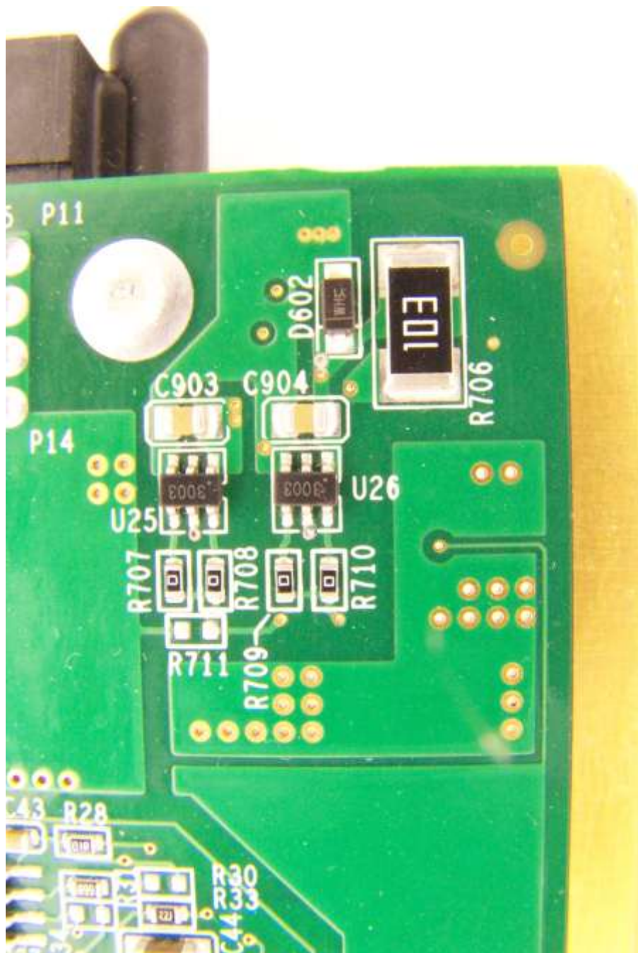
Photograph 35. PS components 1
