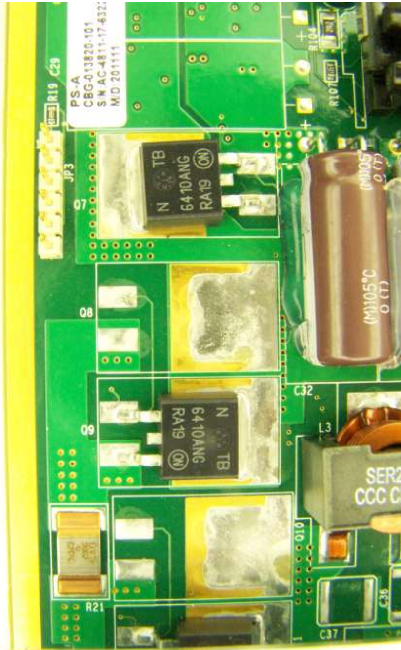
Photograph 46. PS components 12
