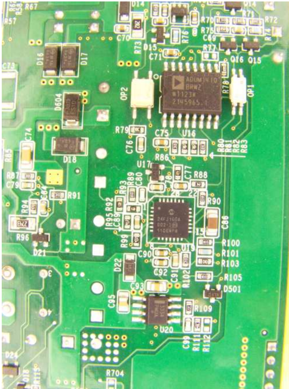
Photograph 39. PS components 5
