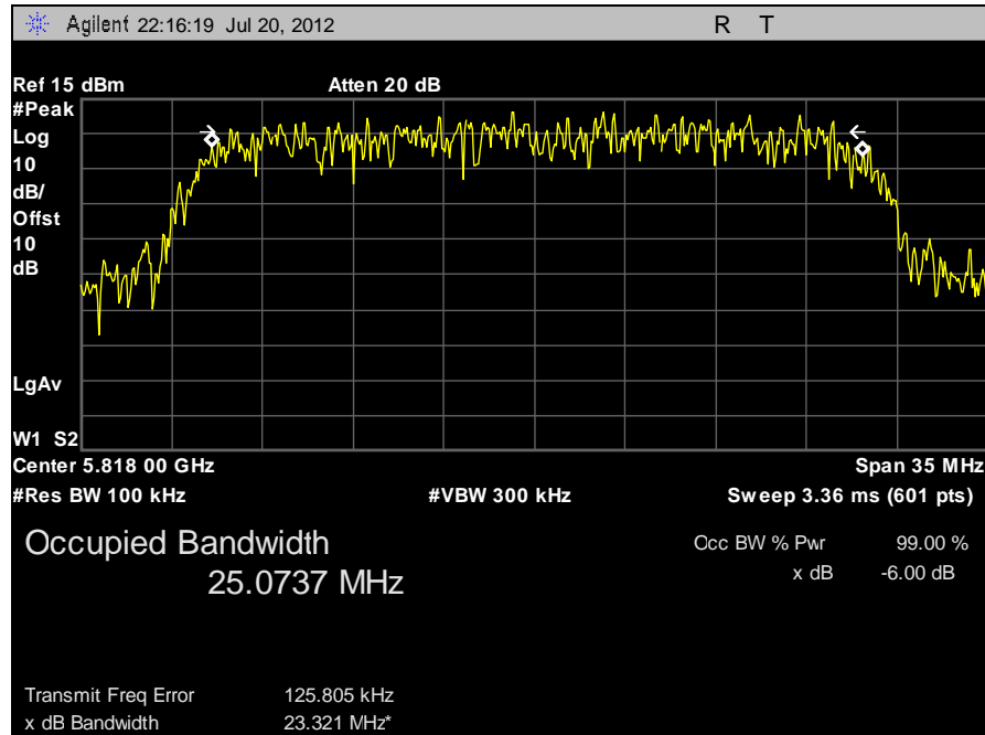
Plot 5. 6 dB Occupied Bandwidth, 5818 MHz
