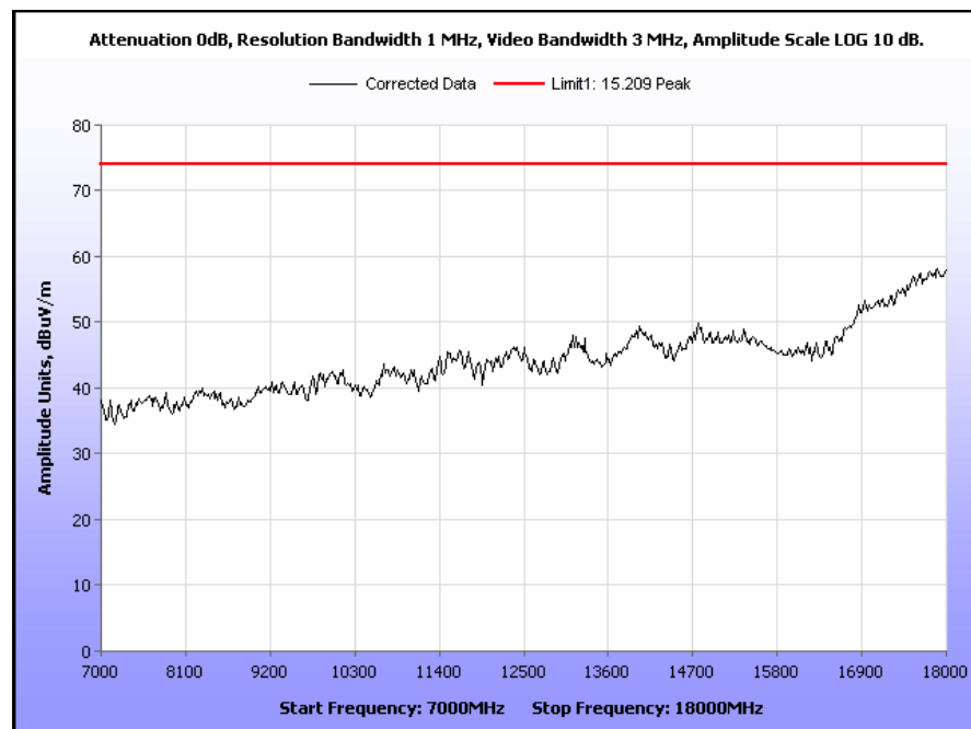
Plot 24. Radiated Spurious Emissions, 5818 MHz, 7 GHz – 18 GHz, Peak
