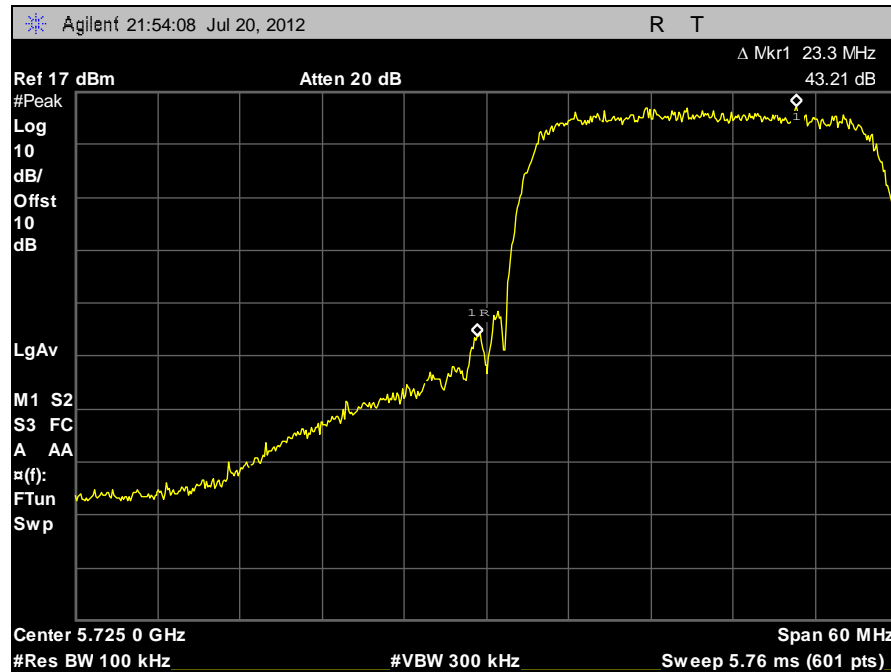
Plot 39. Conducted Spurious Emissions, 5741 MHz, Band Edge
