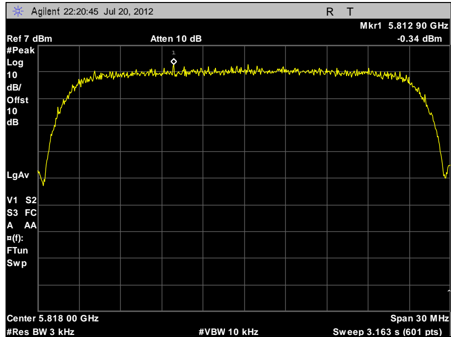
Plot 45. Peak Power Spectral Density, 5818 MHz, Peak Determination
