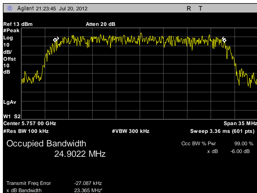
Plot 4. 6 dB Occupied Bandwidth, 5757 MHz
