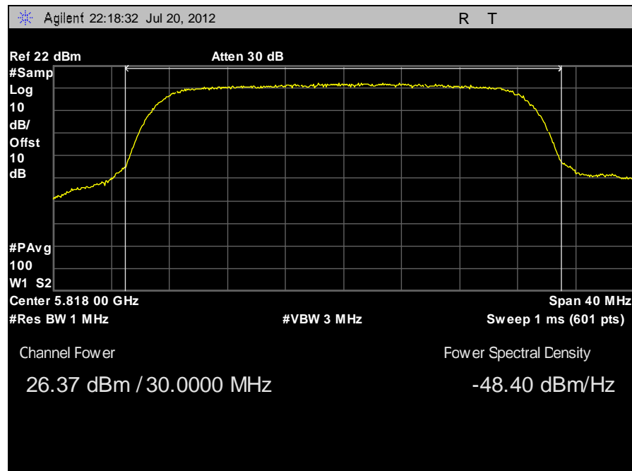
Plot 9. Peak Power Output, 5818 MHz
