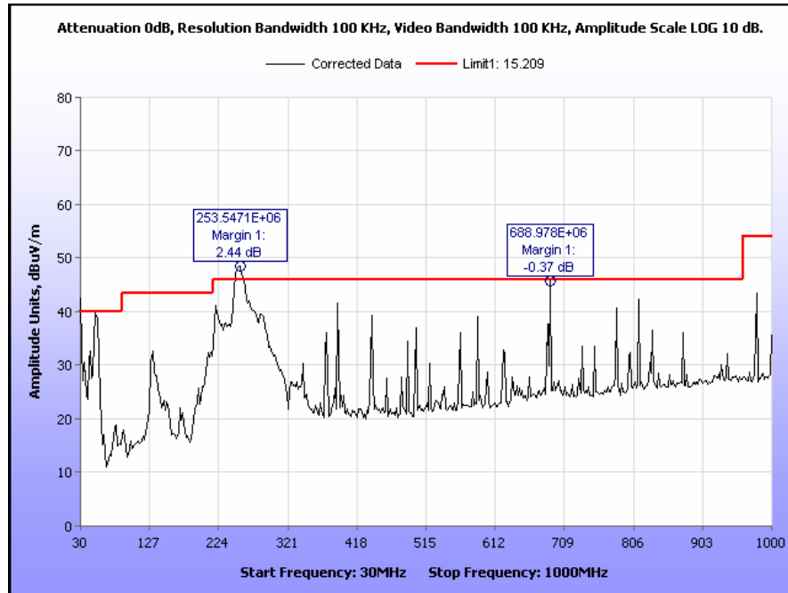
Plot 21. Radiated Spurious Emissions, 5818 MHz, 30 MHz – 1 GHz
