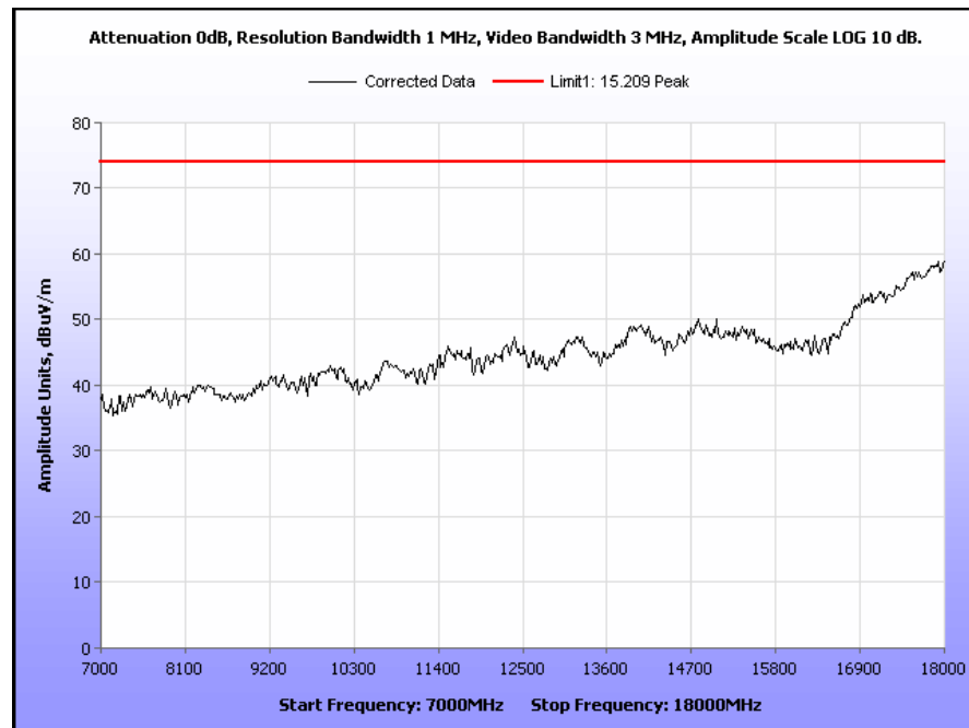
Plot 14. Radiated Spurious Emissions, 5741 MHz, 7 GHz – 18 GHz, Peak
