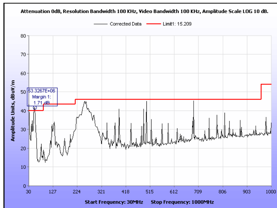
Plot 16. Radiated Spurious Emissions, 5757 MHz, 30 MHz – 1 GHz
