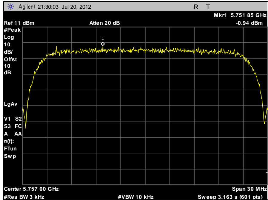
Plot 43. Peak Power Spectral Density, 5757 MHz, Peak Determination
