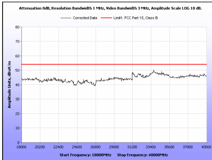
Plot 25. Radiated Spurious Emissions, 5818 MHz, 18 GHz – 40 GHz, Peak under Average
