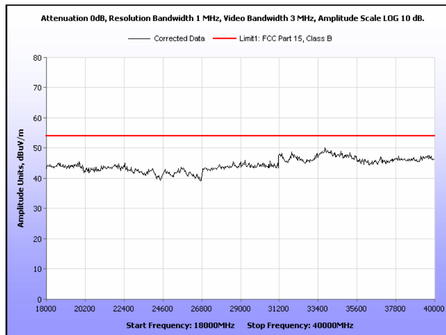
Plot 20. Radiated Spurious Emissions, 5757 MHz, 18 GHz – 40 GHz, Peak under Average
