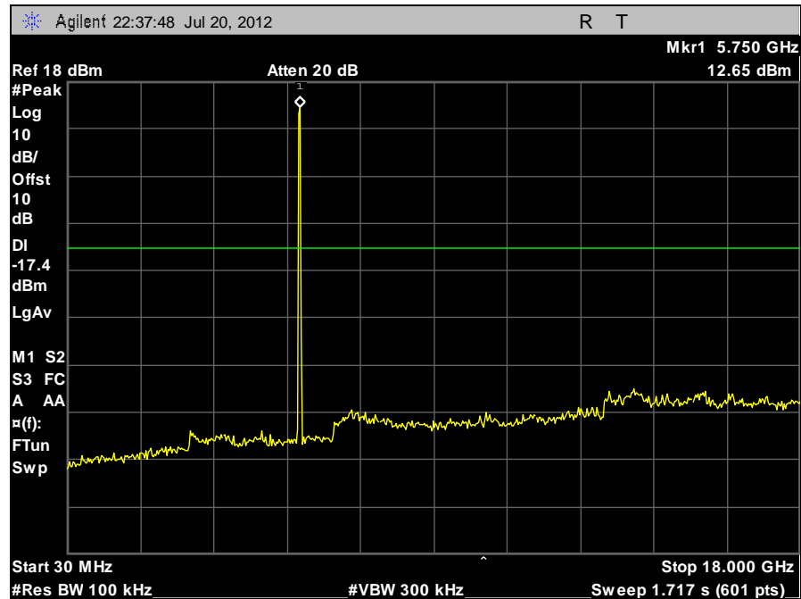
Plot 31. Conducted Spurious Emissions, 5741 MHz, 30 MHz – 18 GHz
