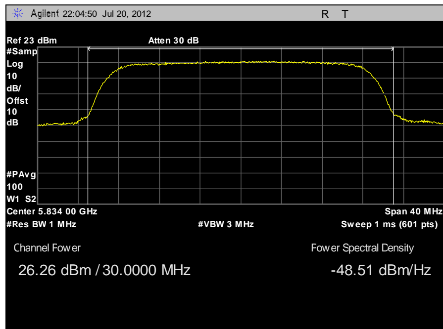
Plot 10. Peak Power Output, 5834 MHz
