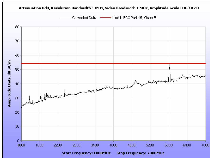
Plot 22. Radiated Spurious Emissions, 5818 MHz, 1 GHz – 7 GHz
