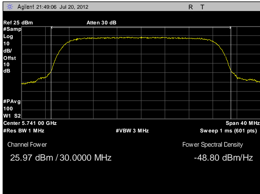
Plot 7. Peak Power Output, 5741 MHz
