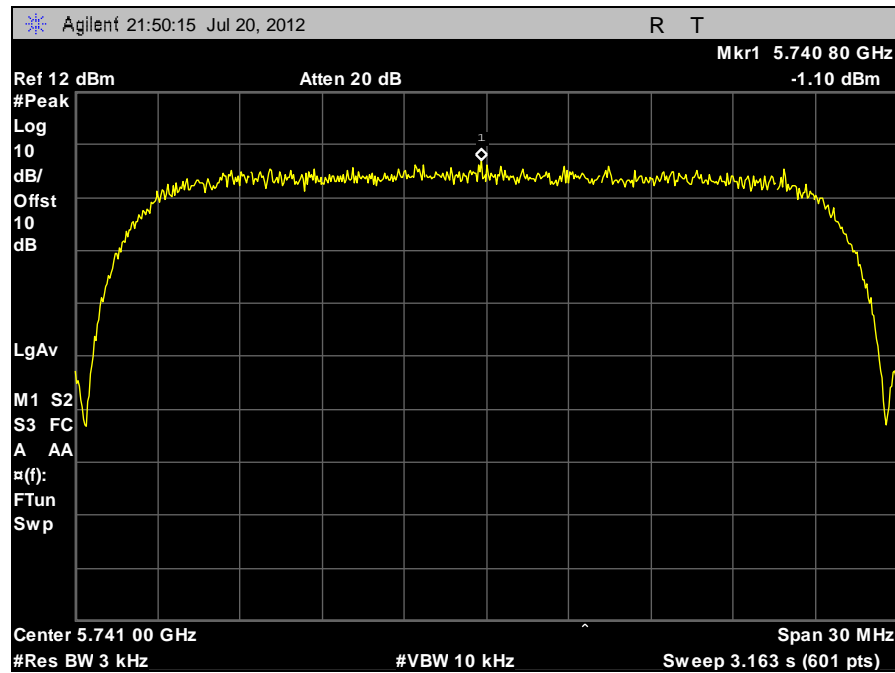
Plot 41. Peak Power Spectral Density, 5741 MHz, Peak Determination
