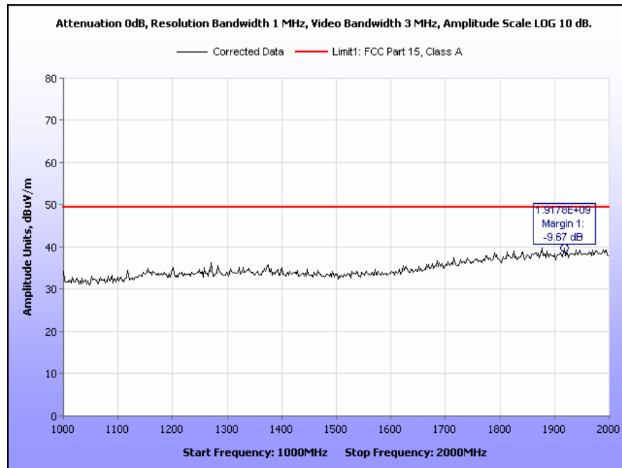
Plot 2. Radiated Emissions, Above 1 GHz, FCC Limits
