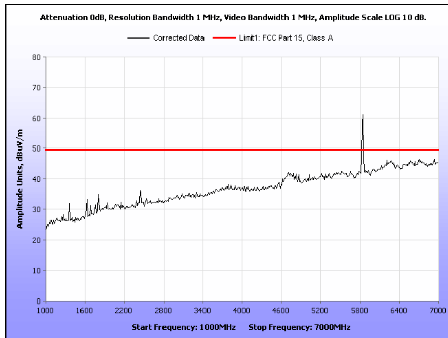
Plot 27. Radiated Spurious Emissions, 5834 MHz, 1 GHz – 7 GHz
