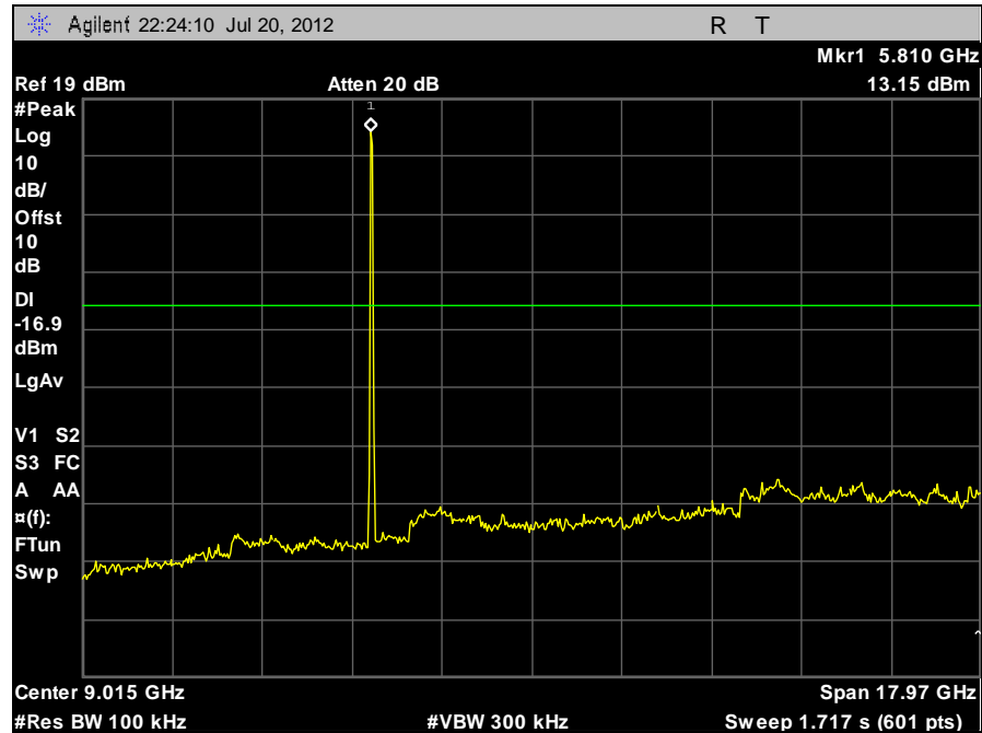
Plot 35. Conducted Spurious Emissions, 5818 MHz, 30 MHz – 18 GHz
