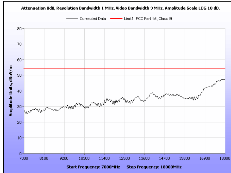
Plot 13. Radiated Spurious Emissions, 5741 MHz, 7 GHz – 18 GHz, Average
