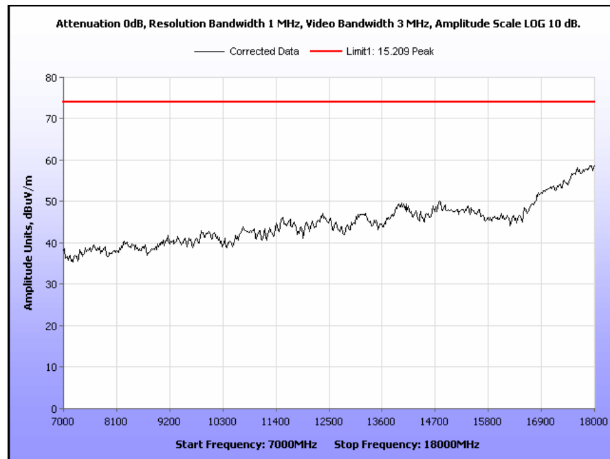
Plot 19. Radiated Spurious Emissions, 5757 MHz, 7 GHz – 18 GHz, Peak
