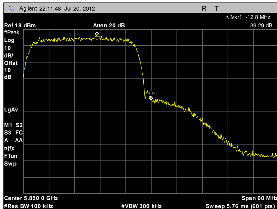
Plot 40. Conducted Spurious Emissions, 5834 MHz, Band Edge
