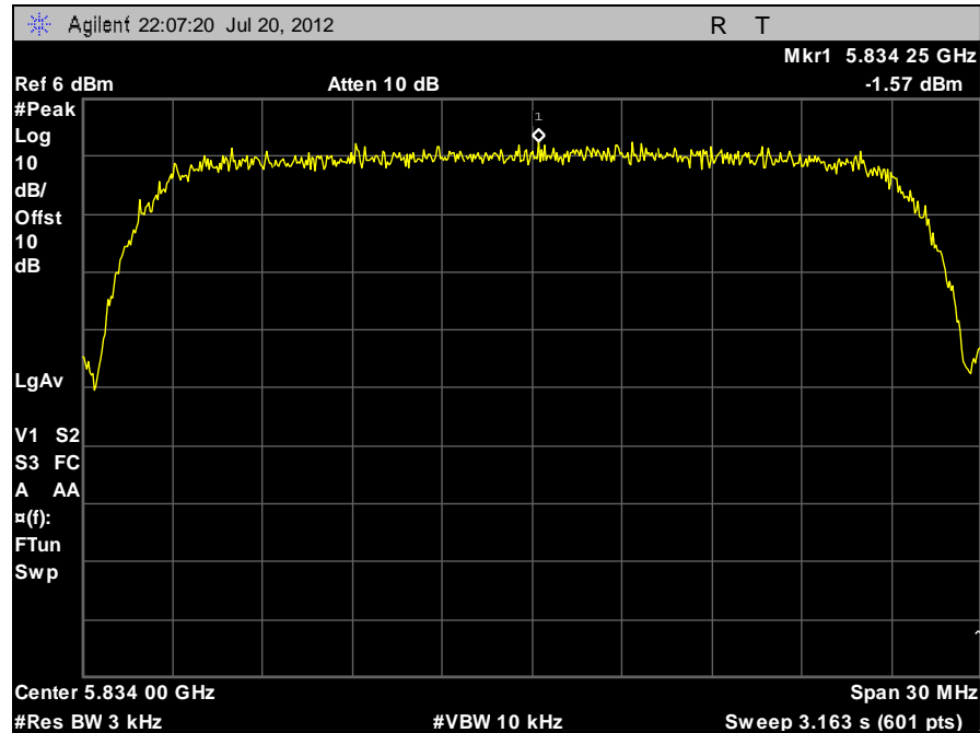
Plot 47. Peak Power Spectral Density, 5834 MHz, Peak Determination
