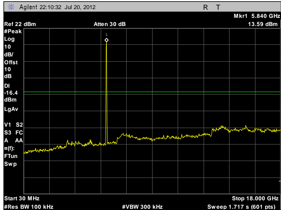
Plot 37. Conducted Spurious Emissions, 5834 MHz, 30 MHz – 18 GHz
