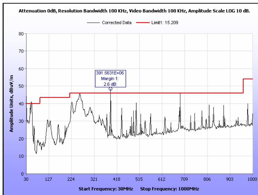
Plot 11. Radiated Spurious Emissions, 30 MHz – 1 GHz
