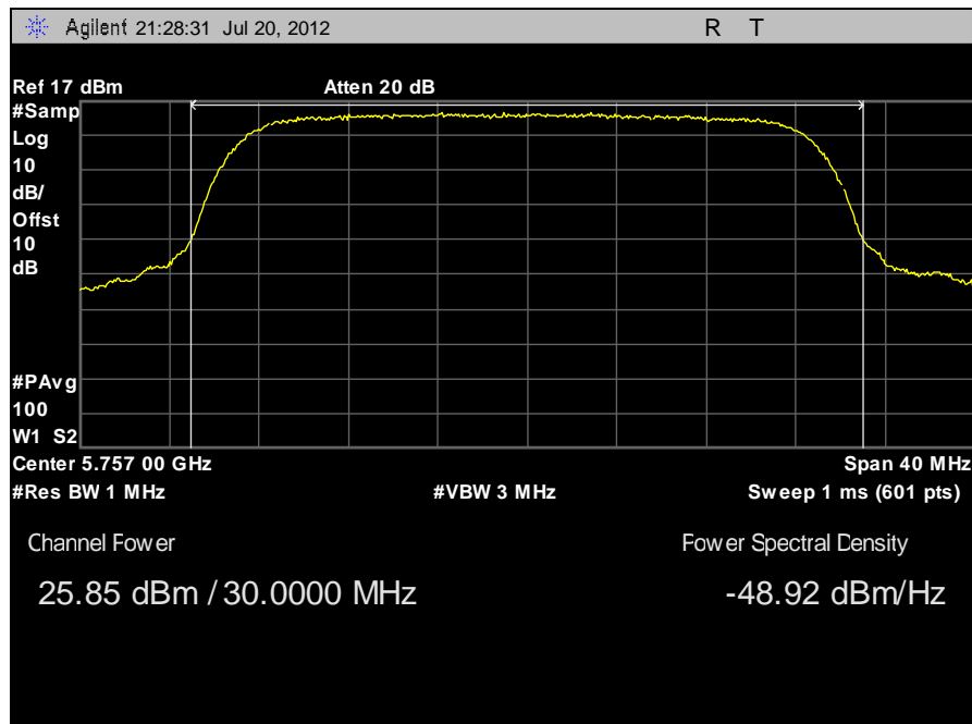
Plot 8. Peak Power Output, 5757 MHz
