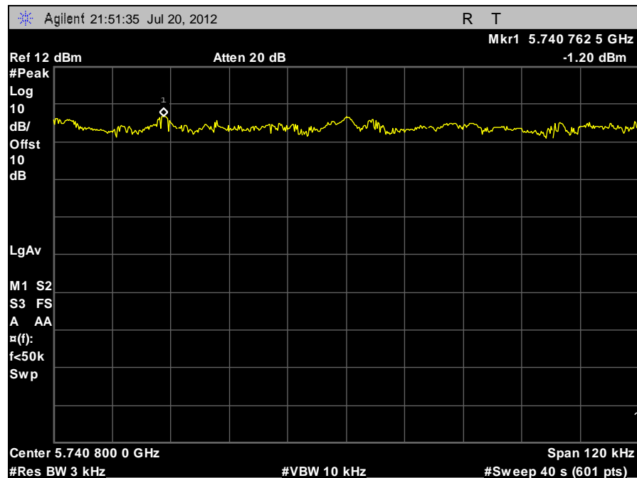
Plot 42. Peak Power Spectral Density, 5741 MHz
