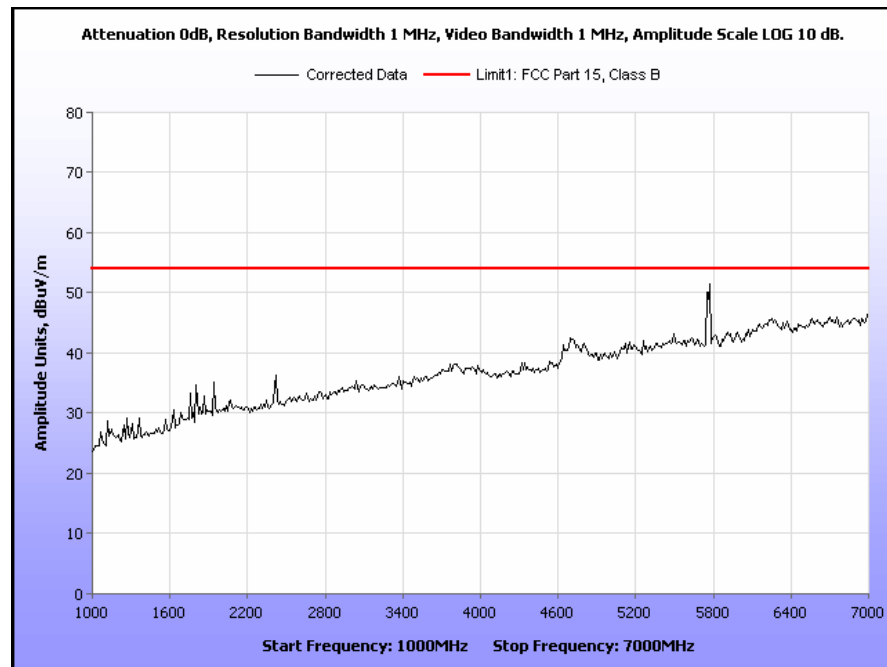
Plot 17. Radiated Spurious Emissions, 5757 MHz, 1 GHz – 7 GHz
