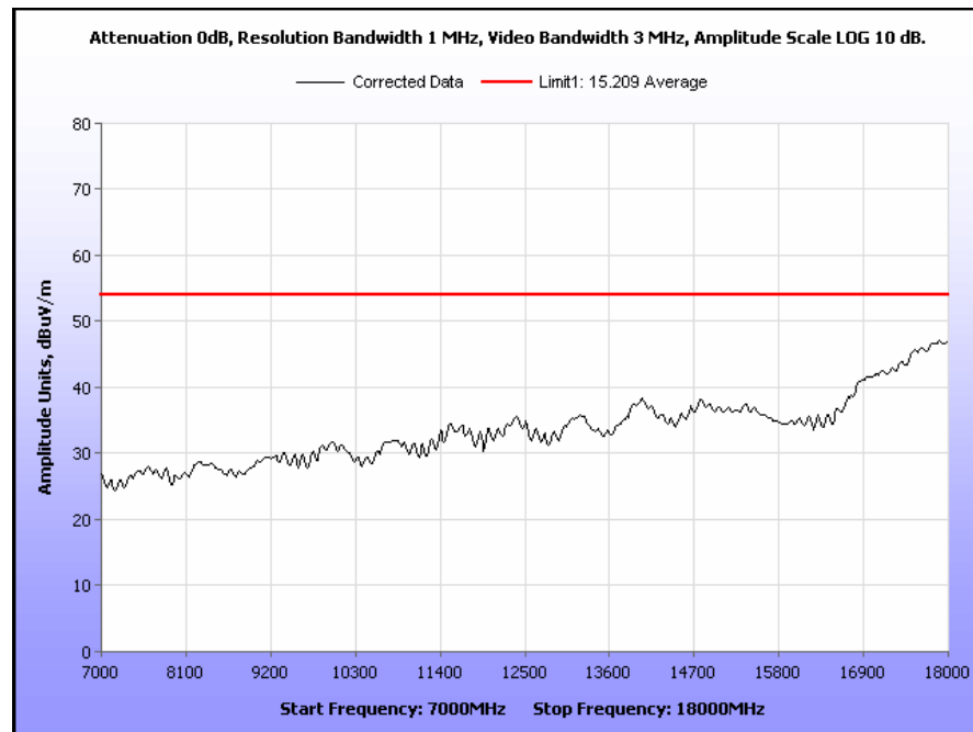
Plot 23. Radiated Spurious Emissions, 5818 MHz, 7 GHz – 18 GHz, Average
