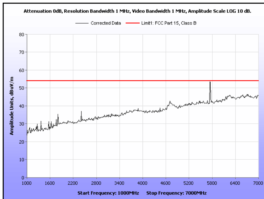
Plot 12. Radiated Spurious Emissions, 1 GHz – 7 GHz
