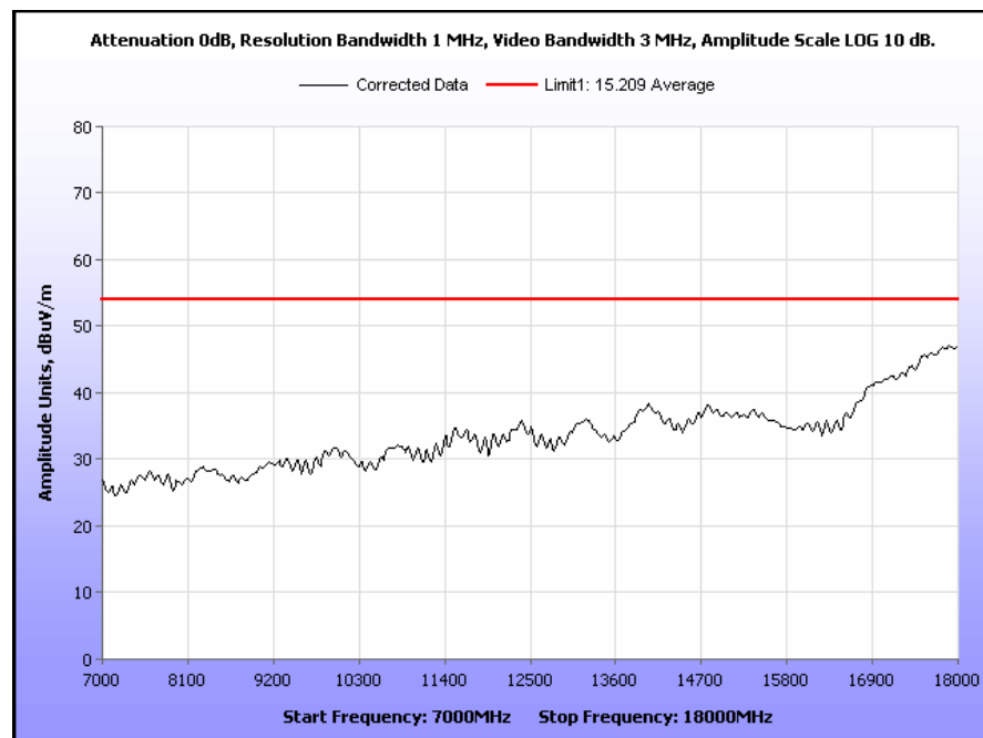
Plot 18. Radiated Spurious Emissions, 5757 MHz, 7 GHz – 18 GHz, Average
