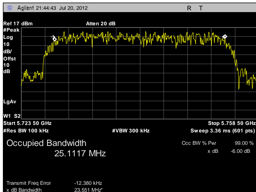
Plot 3. 6 dB Occupied Bandwidth, 5741 MHz
