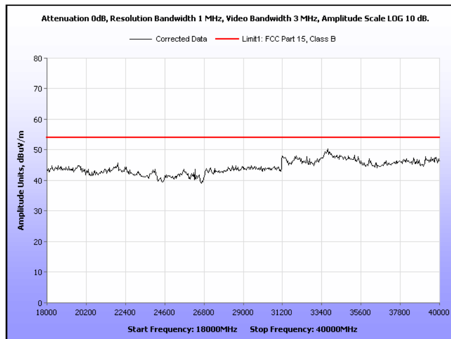
Plot 30. Radiated Spurious Emissions, 5834 MHz, 18 GHz – 40 GHz, Peak under Average
