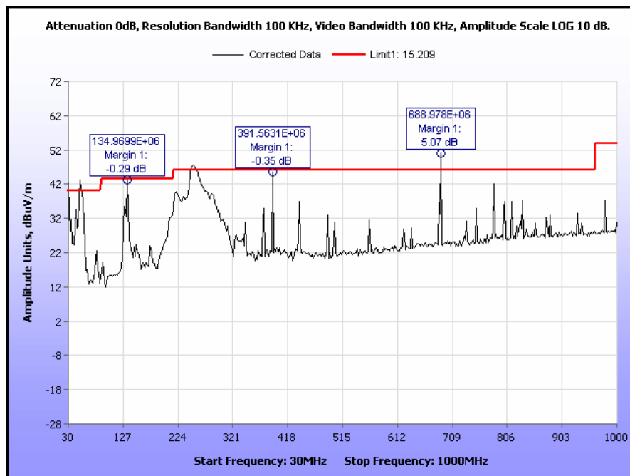
Plot 26. Radiated Spurious Emissions, 5834 MHz, 30 MHz – 1 GHz
