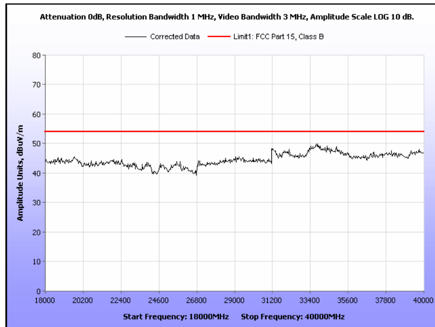
Plot 15. Radiated Spurious Emissions, 5741 MHz, 18 GHz – 40 GHz, Peak under Average
