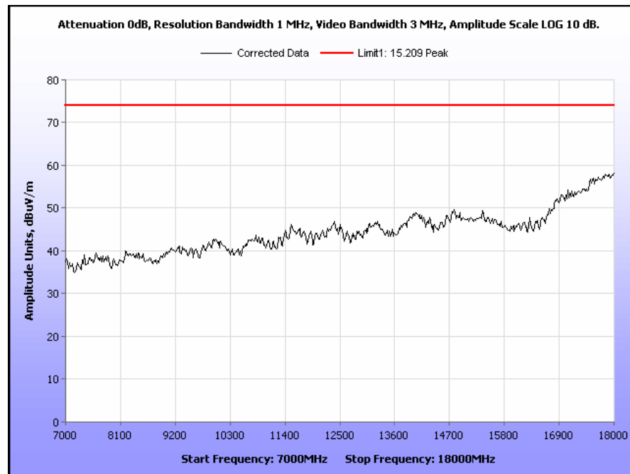
Plot 29. Radiated Spurious Emissions, 5834 MHz, 7 GHz – 18 GHz, Peak
