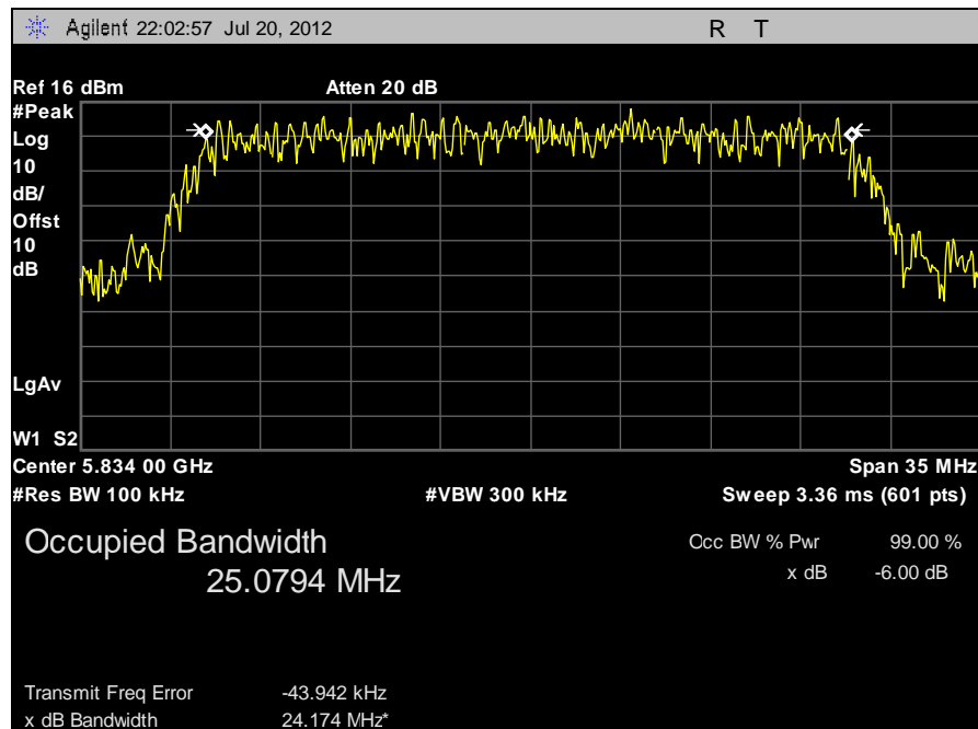
Plot 6. 6 dB Occupied Bandwidth, 5834 MHz
