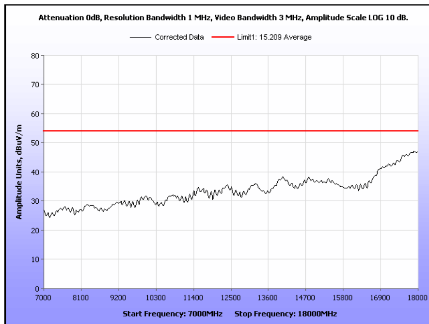
Plot 28. Radiated Spurious Emissions, 5834 MHz, 7 GHz – 18 GHz, Average
