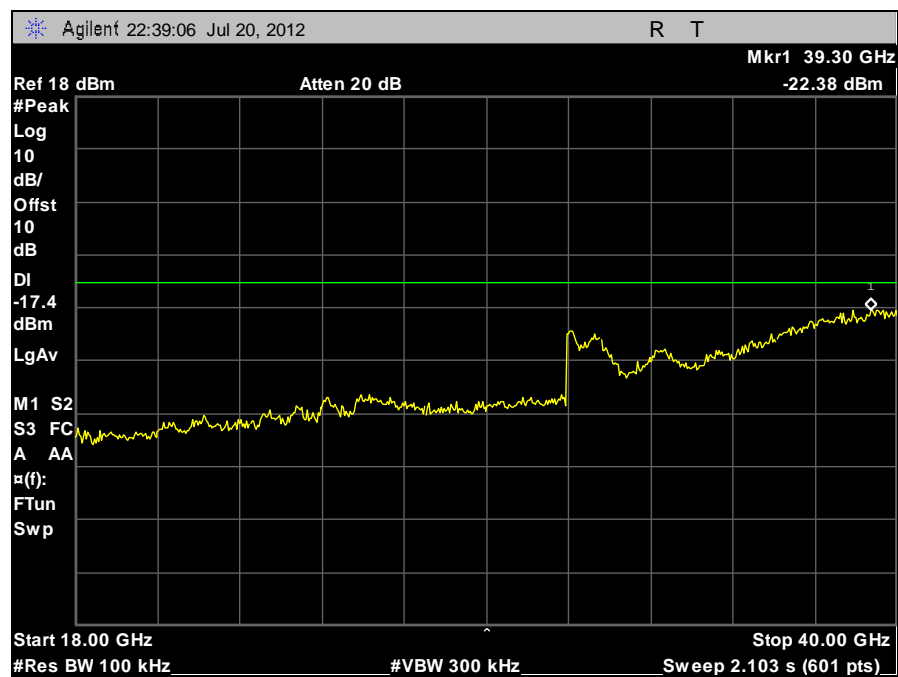
Plot 32. Conducted Spurious Emissions, 5741 MHz, 18 GHz – 40 GHz
