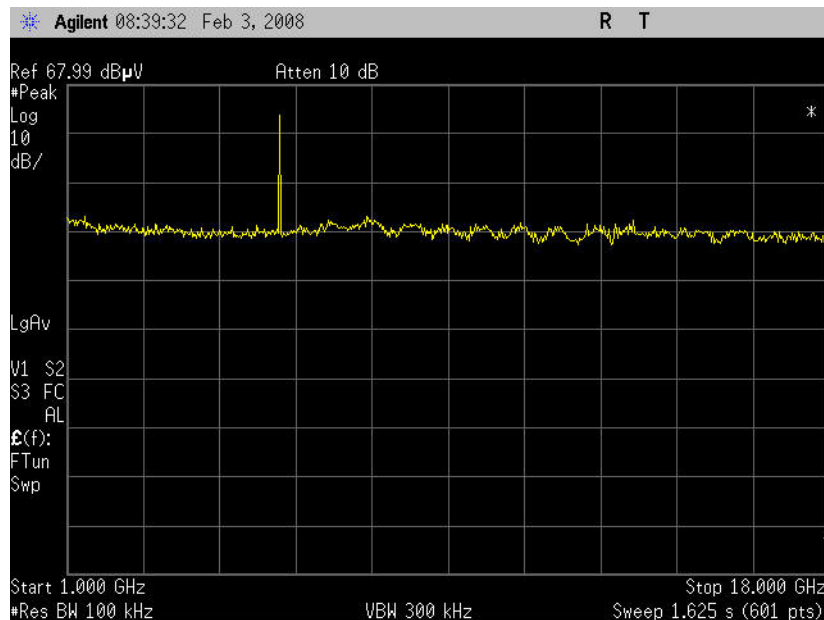
Radiated Spurious Emissions 1-18GHz Low Channel
