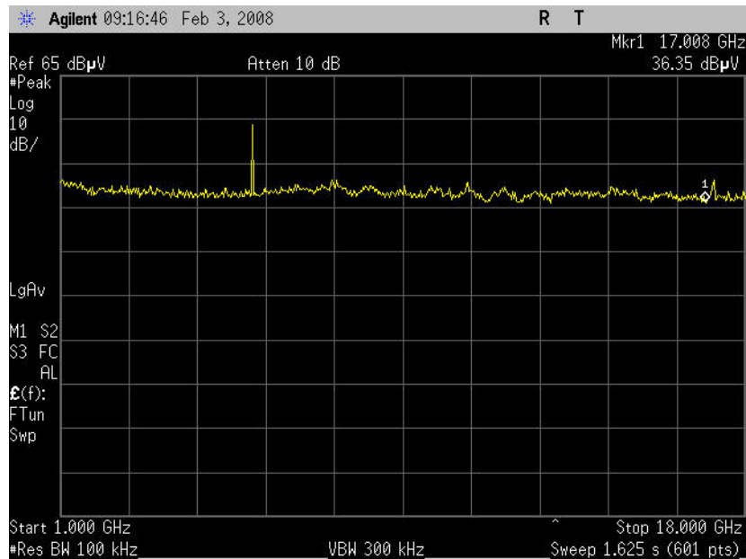
Radiated Spurious Emissions 1-18GHz Mid Channel
