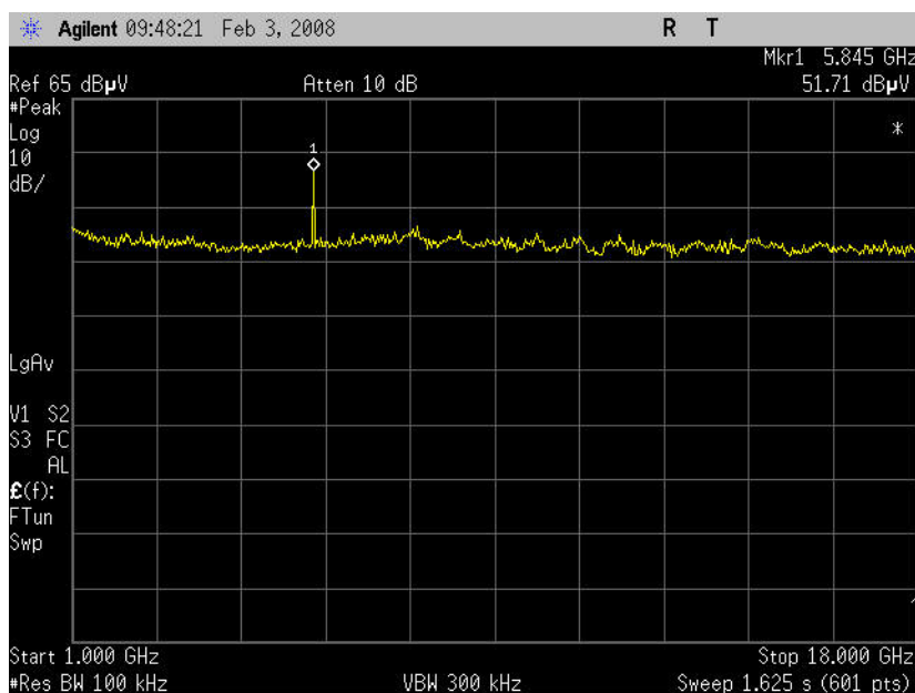
Radiated Spurious Emissions 1-18GHz High Channel
