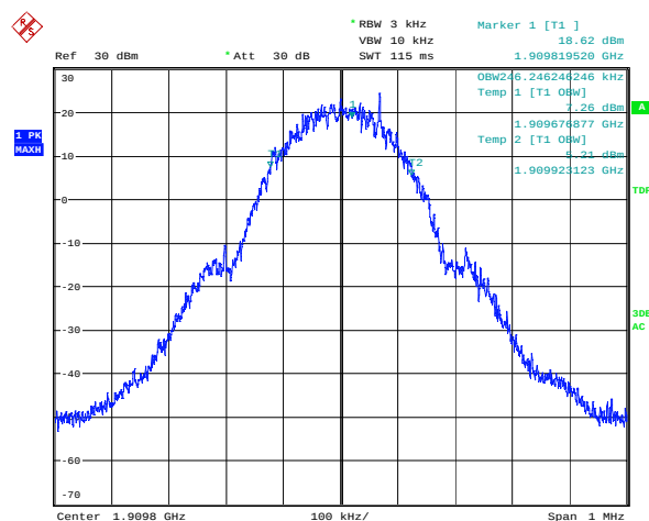
Occupied Bandwidth (810ch)
