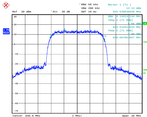
4233ch Occupied Bandwidth (HSDPA)
