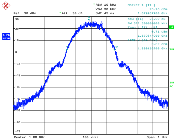
26dB Bandwidth (661ch)
