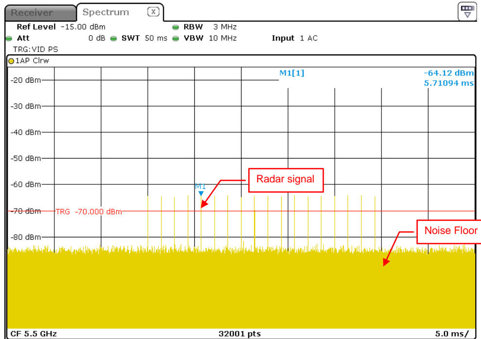
Radar Signal 0
