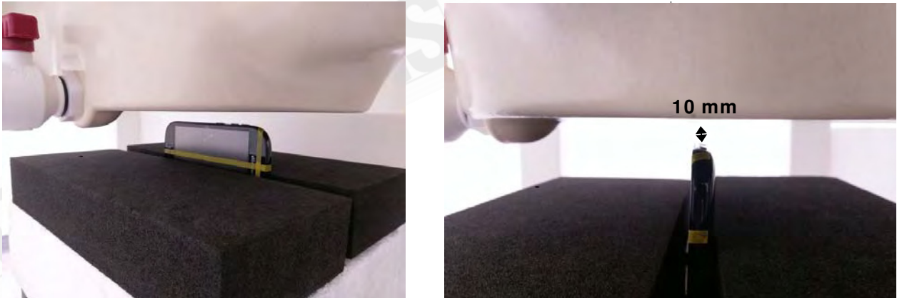
Fig.13 EUT Left side to flat phantom
