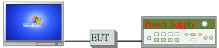
Fig 2-2 Conducted (Antenna Port) Emission Configuration
