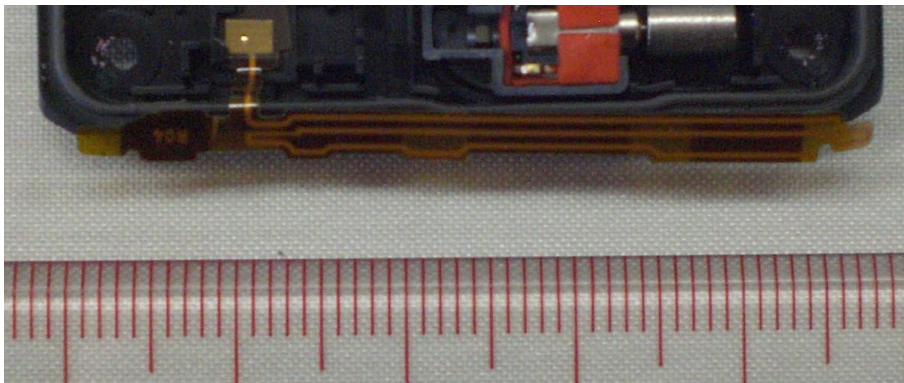
BT/WLAN Antenna
