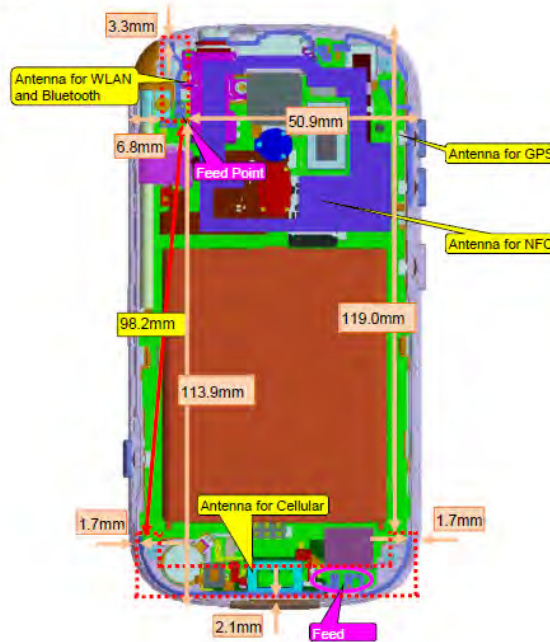
F-03K Antenna Position Back Side
