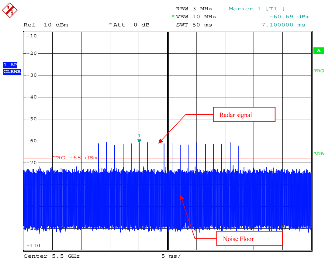
Radar Signal 1
