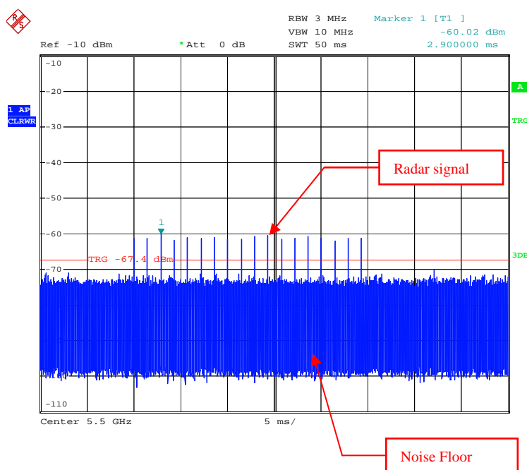
Radar Signal 1
