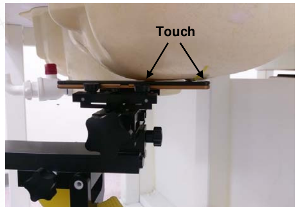
Fig.5 Left Head Section / Cheek-Touch Position
