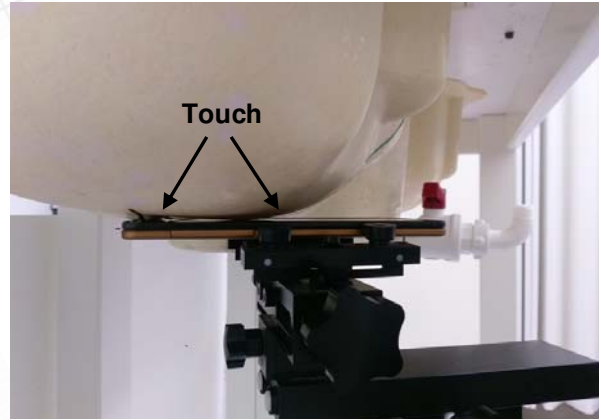
Fig.3 Right Head Section / Cheek-Touch Position
