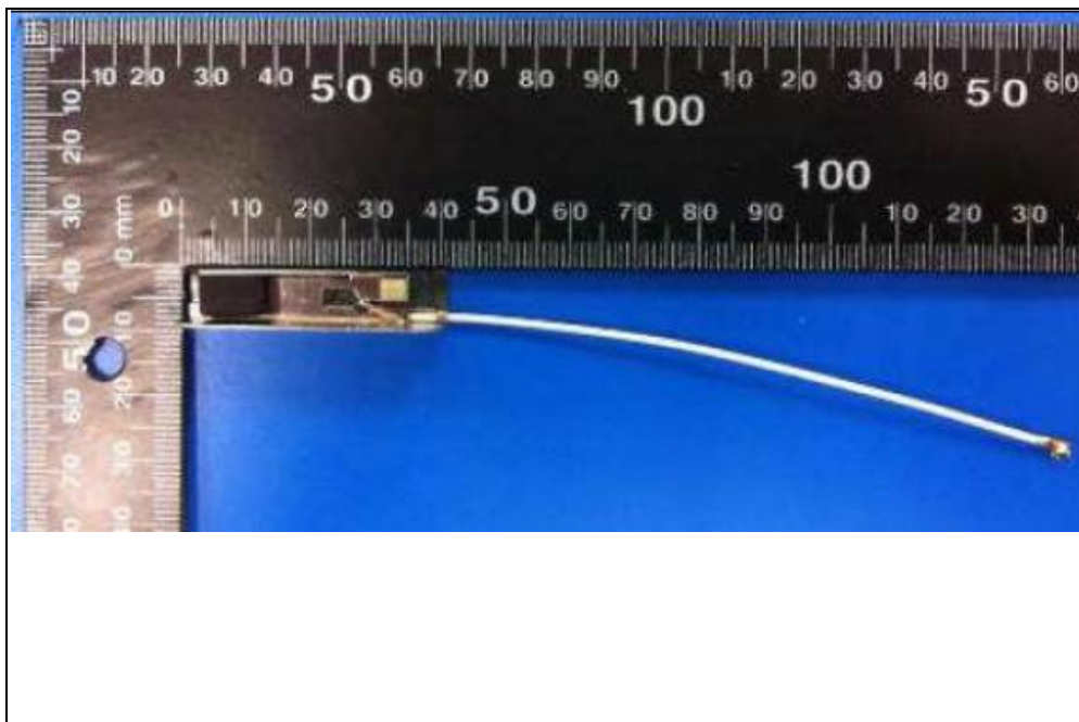
Antenna 96 PIFA Antenna (Brand name: WNC, Model No.: 81.EZY15.GAN/ 25.91458.001)
