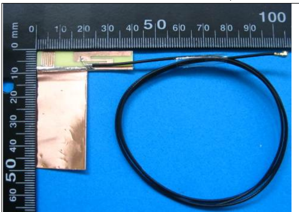
Antenna 116 PIFA Antenna (Brand name: Smart Approach, Model No.: SE-EIPNA-001, SE-EIPNA-002)
