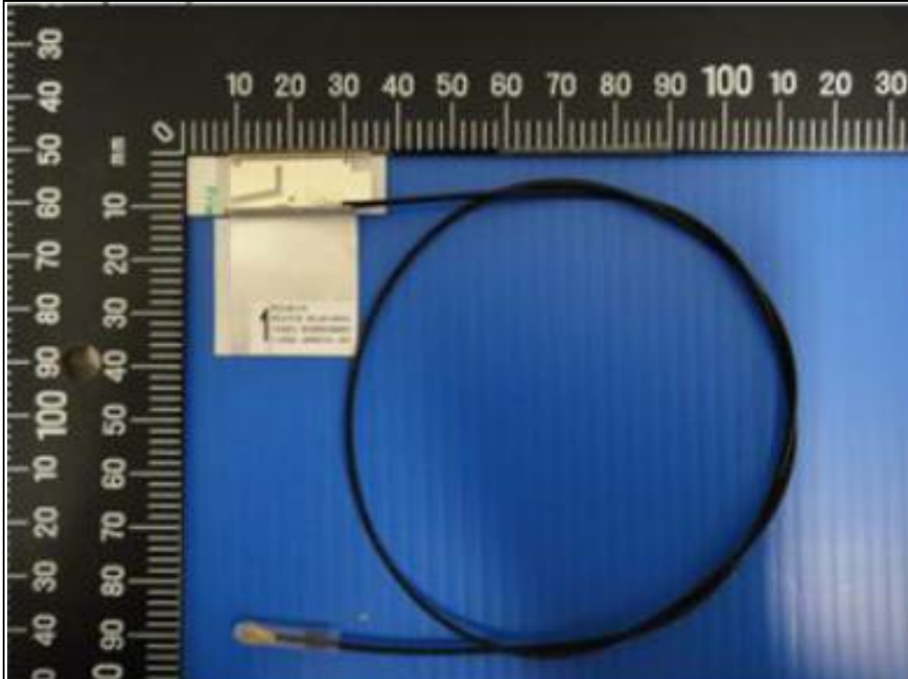
Antenna 105 PIFA Antenna (Brand name: Yageo, Model No.: 6036B0088901/CAN43130LIIN03841)
