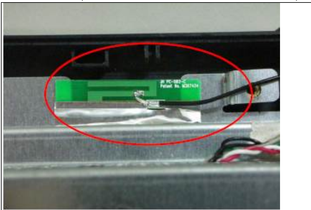
PIFA Antenna (Brand name: Ji-Haw, Model No.: 1415-017J0H2)
