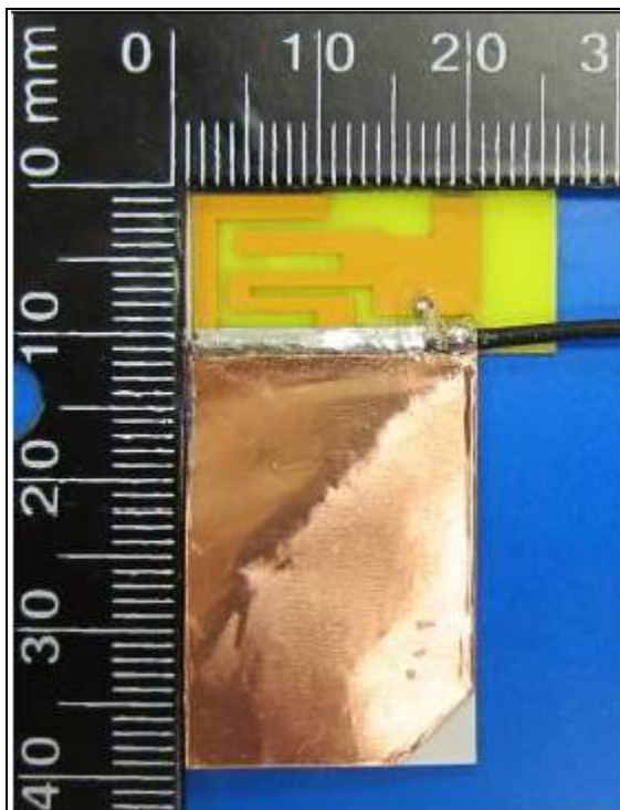
Antenna 74 PIFA Antenna (Brand name: WNC, Model No.: DQ6Y15GCB00 (81.EZY15.GCB), DQ6Y15GCB00 (81.EZY15.GCB))
