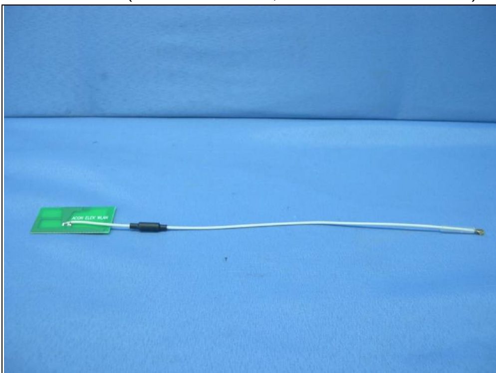
PIFA Antenna (Brand name: ACON, Model No.: APP6P-700119)
