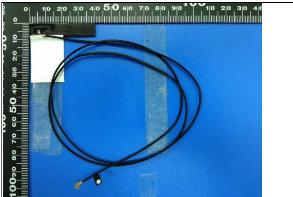
Antenna 117 PIFA Antenna (Brand name: ADVANCED-CONNECTEK INC., Model No.: C-APP6P-700744, C-APP6P-700745)
