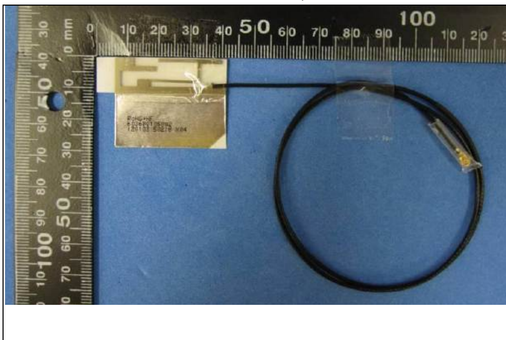
Antenna 93 PIFA Antenna (Brand name: WNC, Model No.: 6036B0105002/ 81.EKT15.G09)
