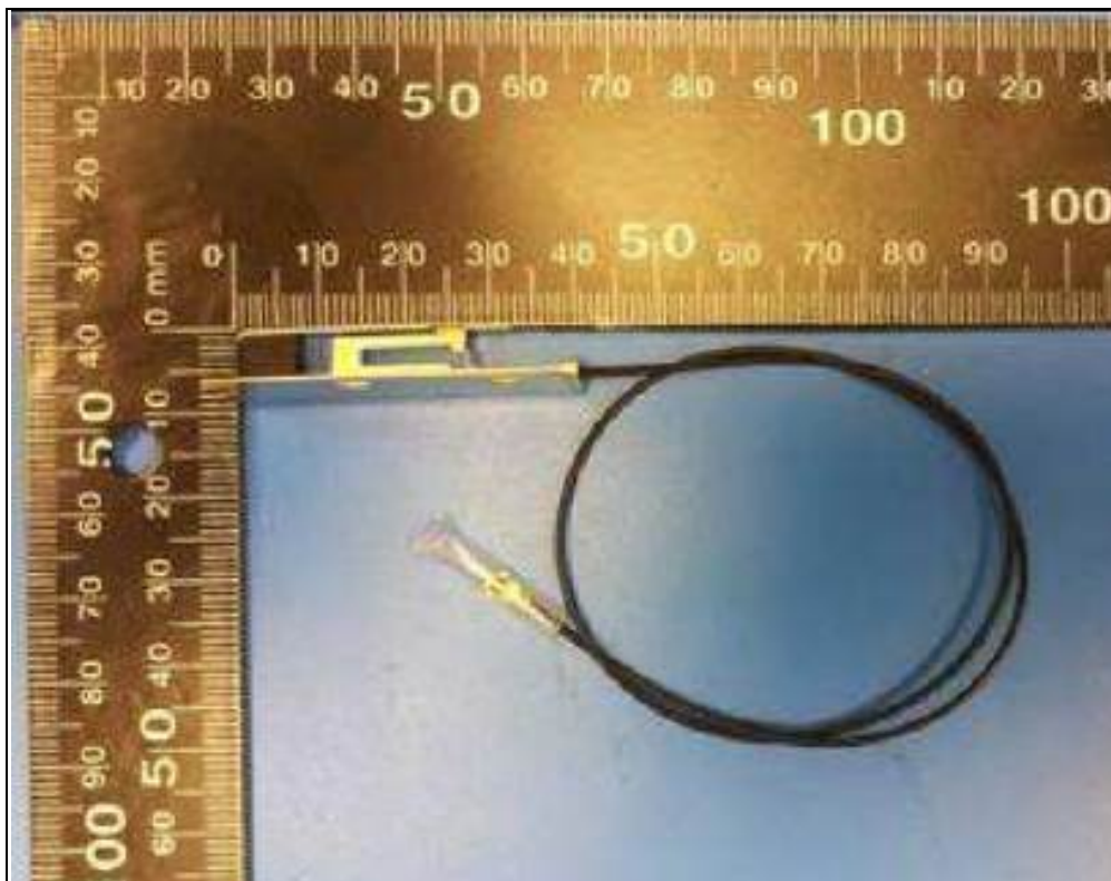
Antenna 82 PIFA Antenna (Brand name: WNC, Model No.: 57.EEW15.0AP, 57XCAE15.030)
