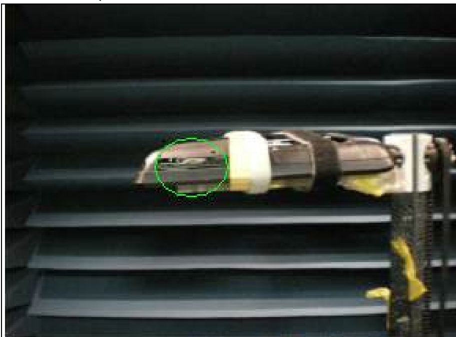
PIFA Antenna (Brand name: WONDERFUL, Model No.: 1415-01DC0H2)
