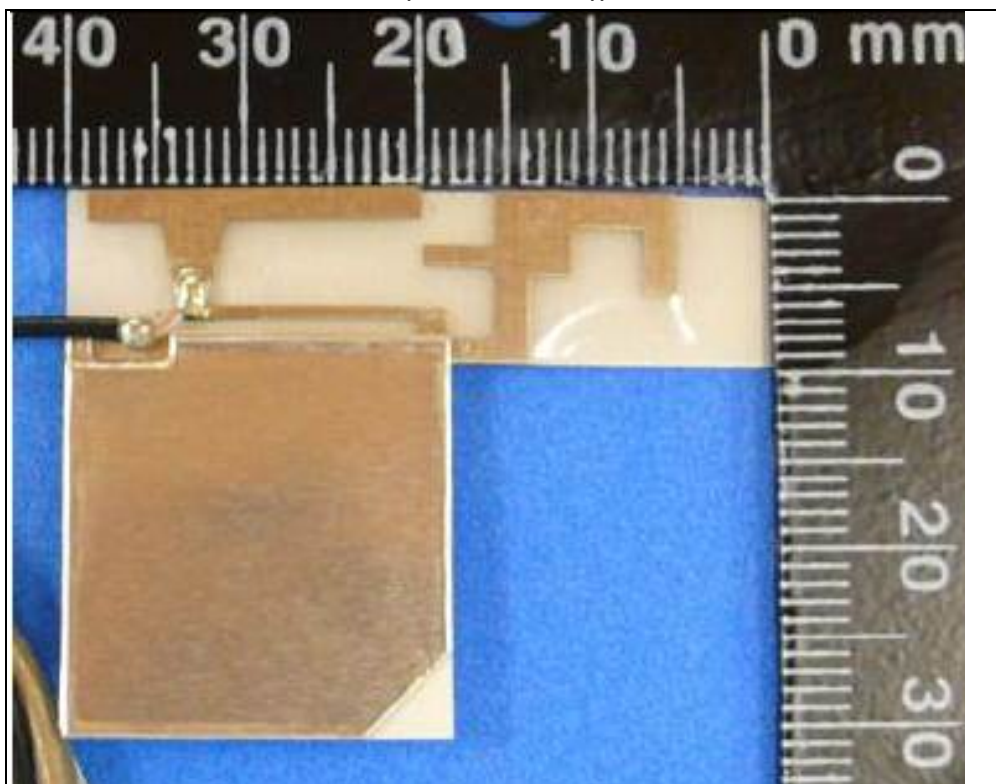
Antenna 97 PIFA Antenna (Brand name: WNC, Model No.: 25.90AEF.001 (81.EL815.G70))
