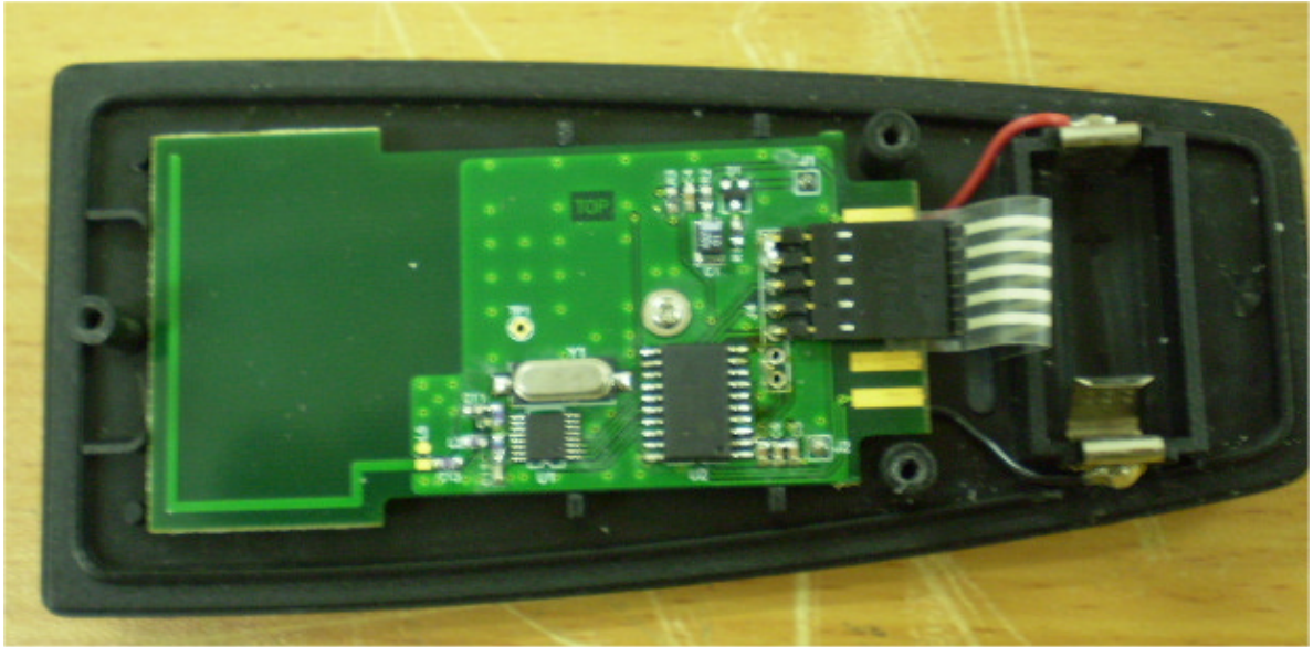
Photograph No.8 RC0100200 remote controller internalview
