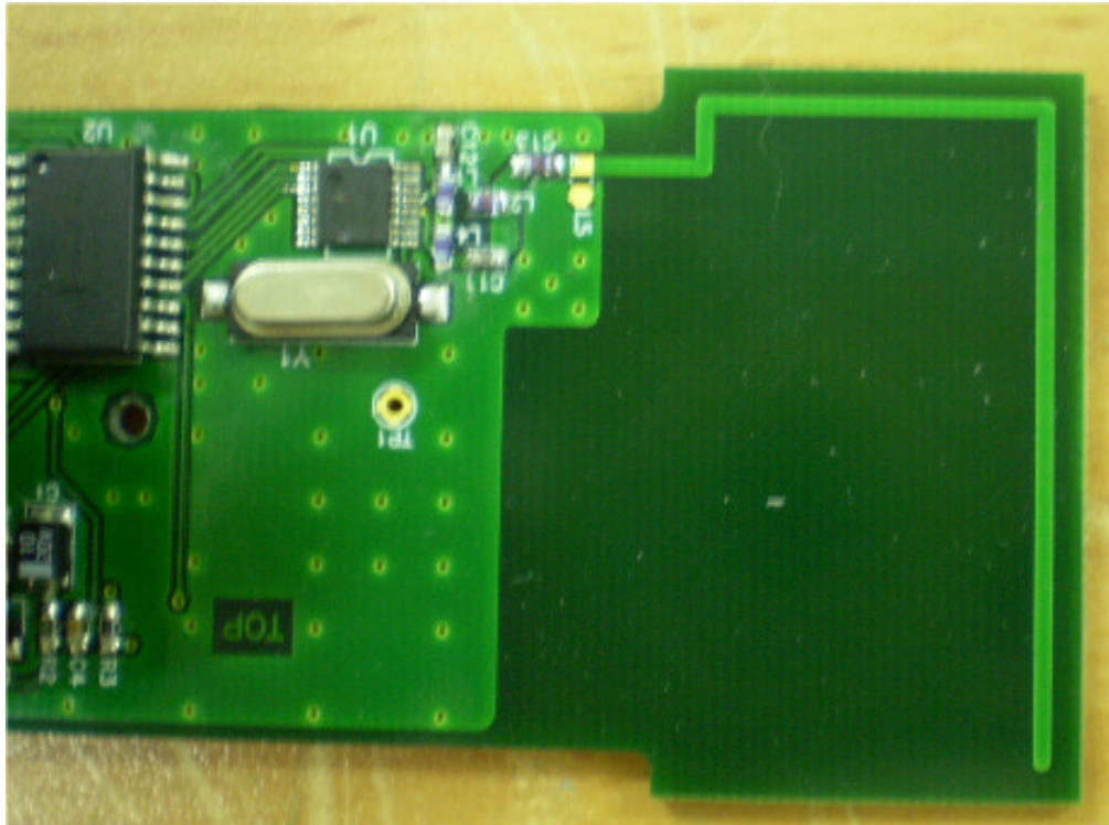
Photograph No.4 RC0100100 remote controller antenna
