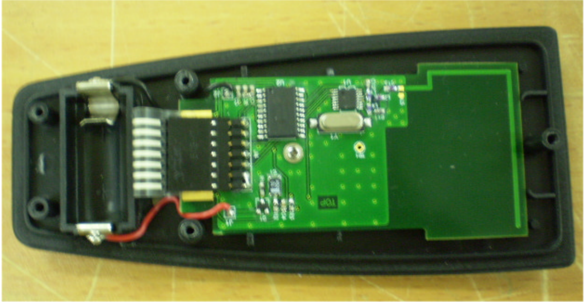
Photograph No.2 RC0100100 remote controller internal view
