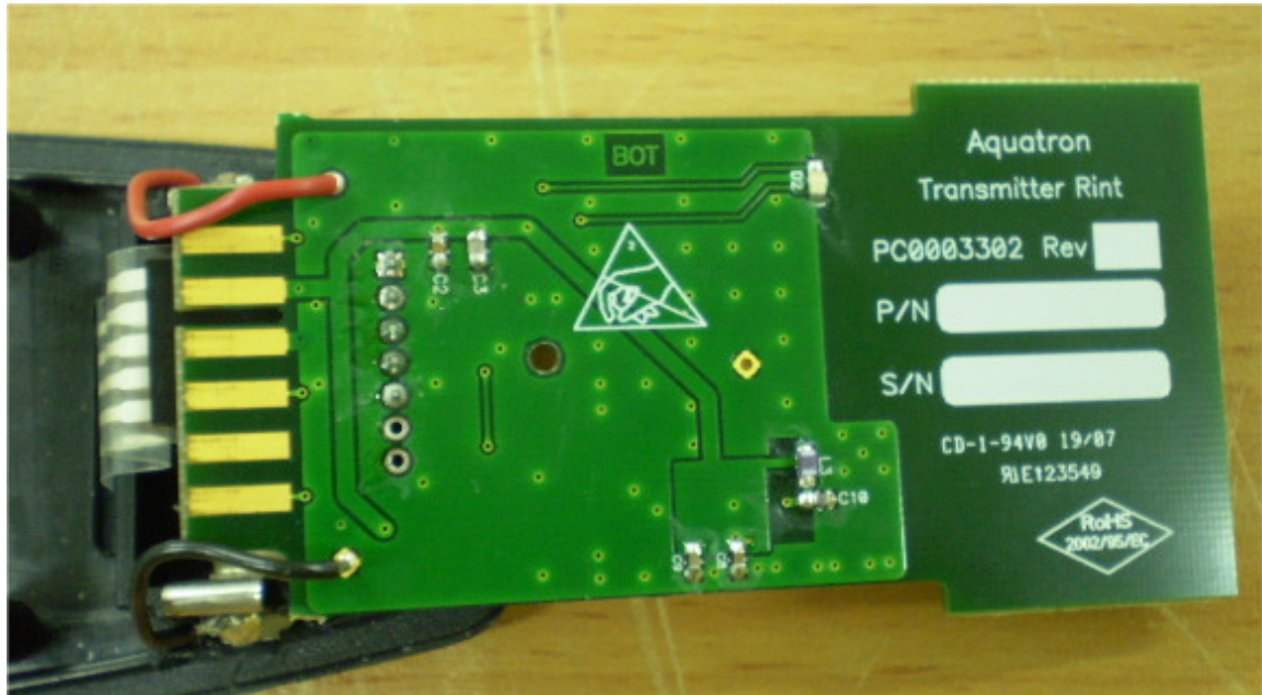
Photograph No.11 RC0100200 remote controller PCB second side view
