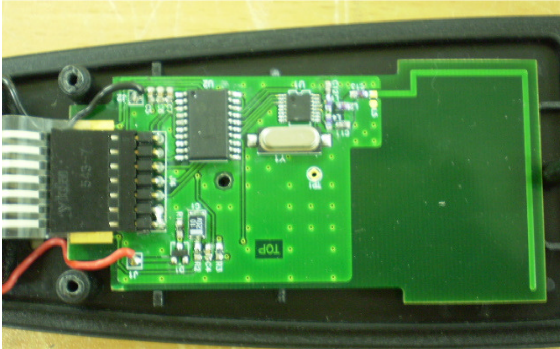
Photograph No.3 RC0100100 remote controller PCB front view
