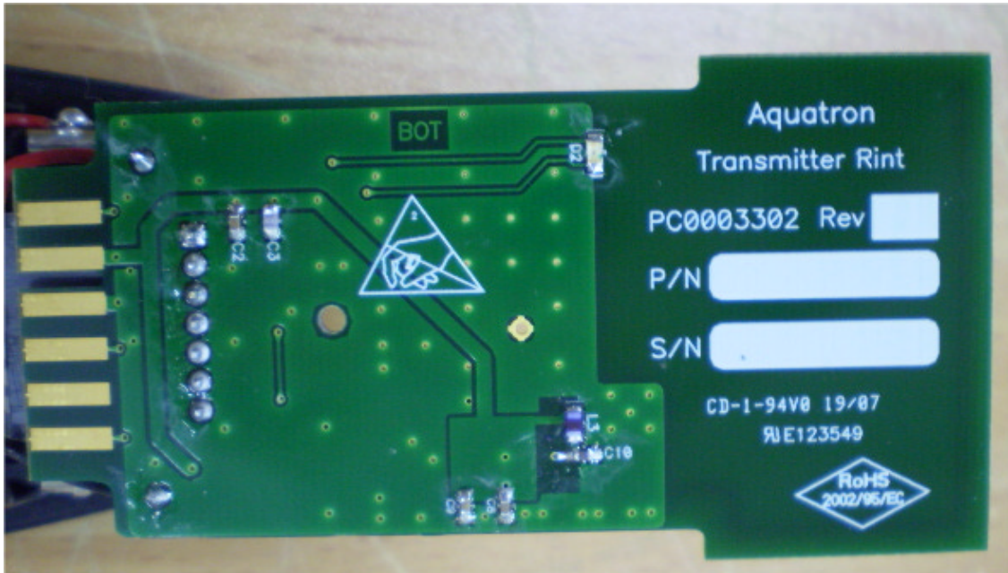
Photograph No.6 PCB second side view
