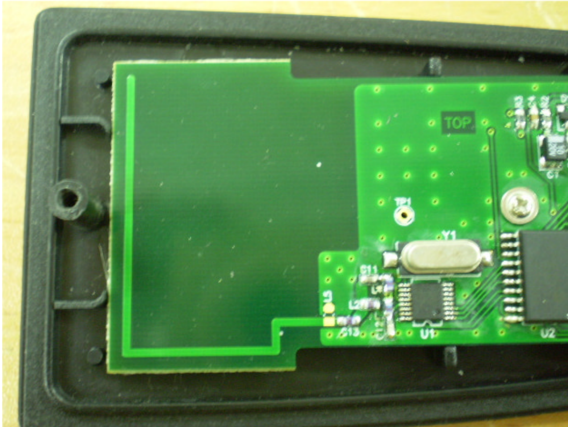
Photograph No.9 RC0100200 remote controller antenna
