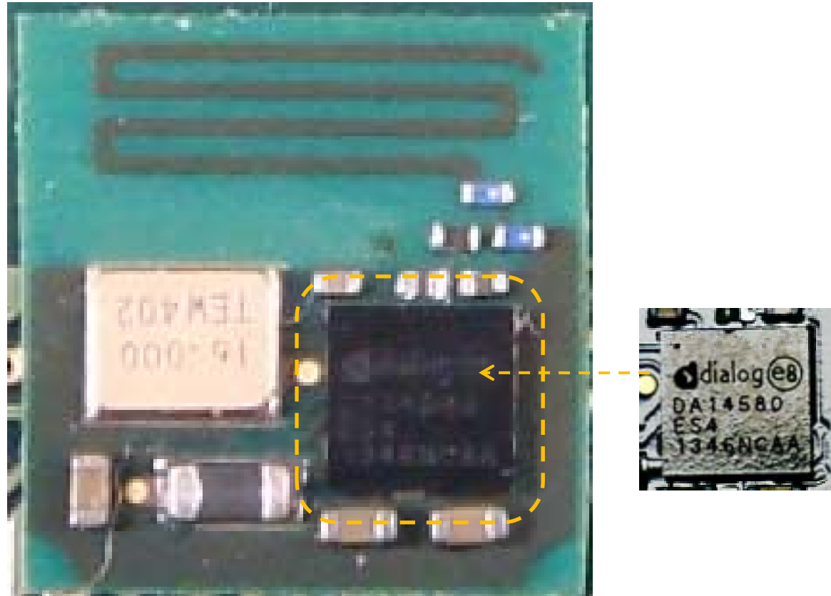
Module(Top --- Unshielded)
