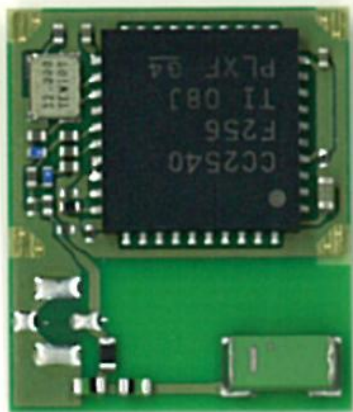
Top View (without metal case)
