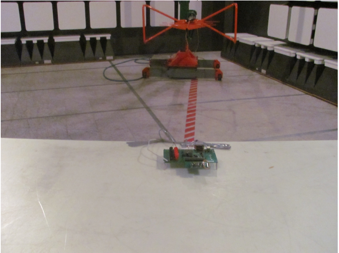
Radiated emissions setup
