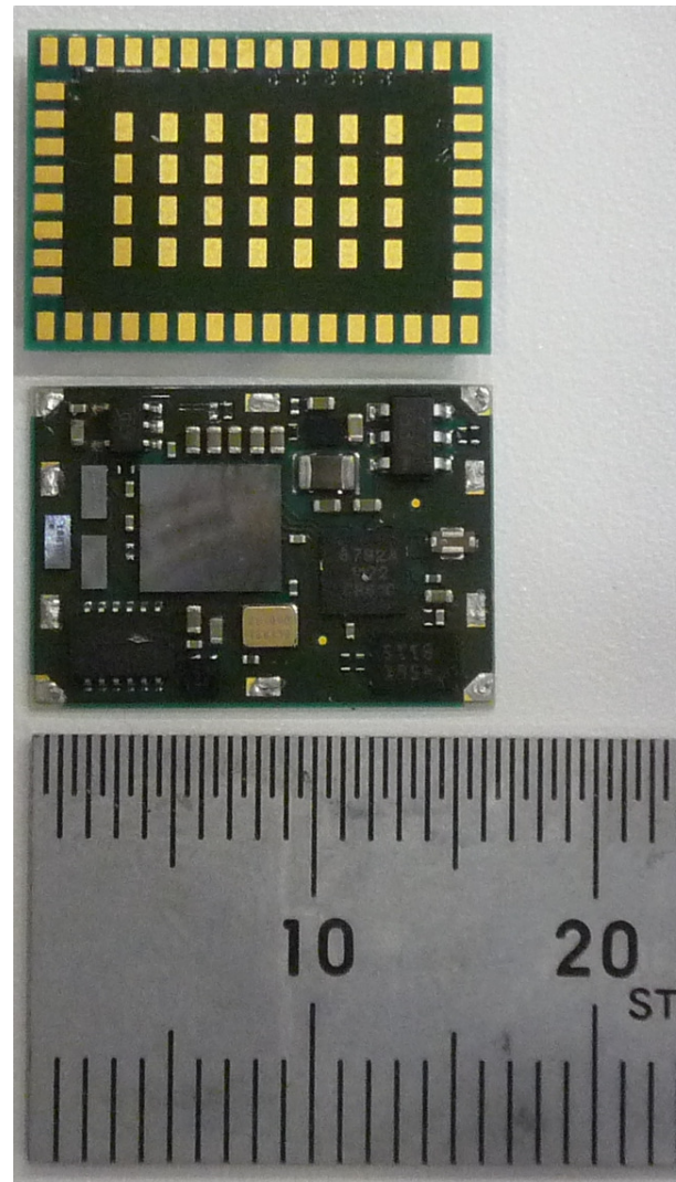
Top View and Bottom View without Shield
