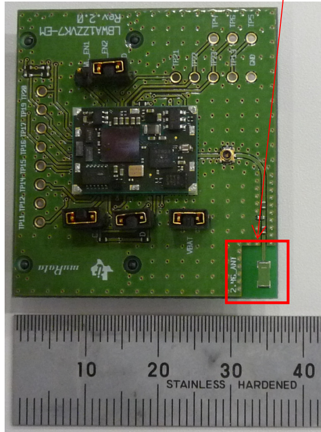
Top View without Shield
