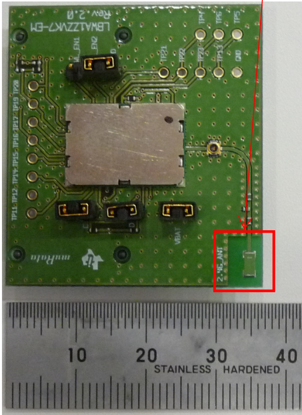
Top View with Shield
