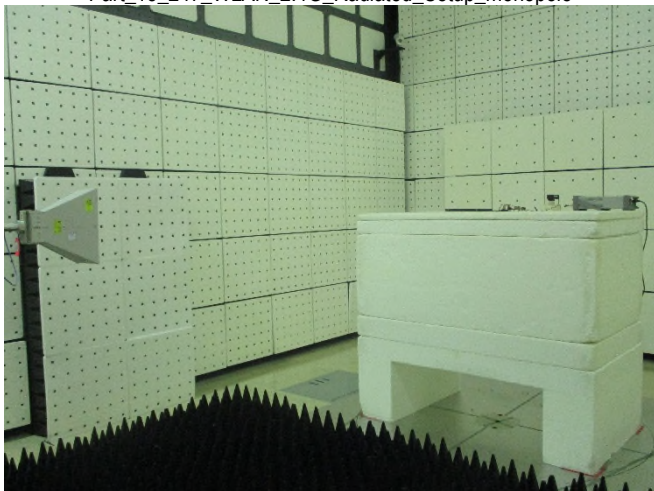
Part_15_247_WLAN_2.4G_Radiated_Setup_monopole
