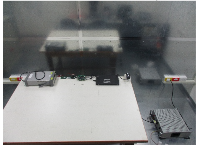
Part_15_247_WLAN_2.4G_Conduction_Setup
