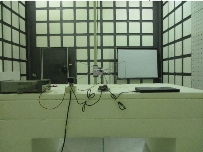
Part_15_247_WLAN_2.4G_Radiated_Setup_dipole
