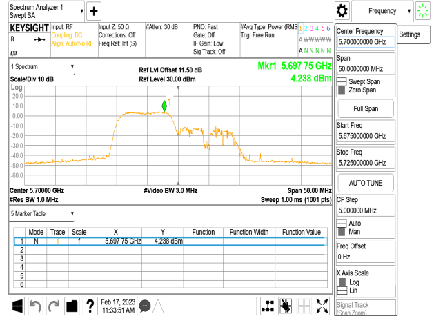
802.11ax_20MHz_Chain0_5700MHz_RU106_54
