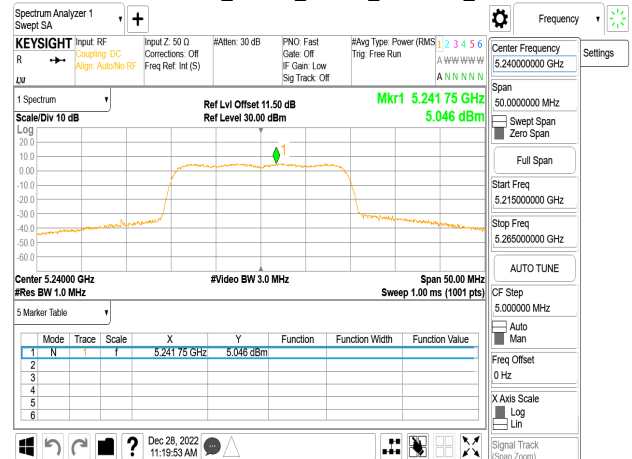
802.11ax_20MHz_Chain0_5240MHz_SU
