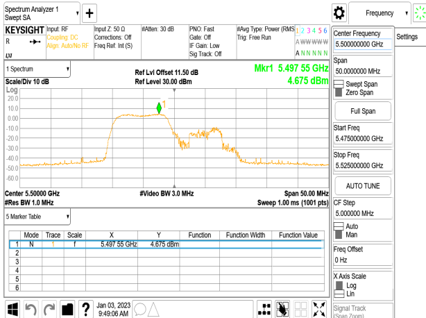
802.11ax_20MHz_Chain0_5500MHz_RU106_54
