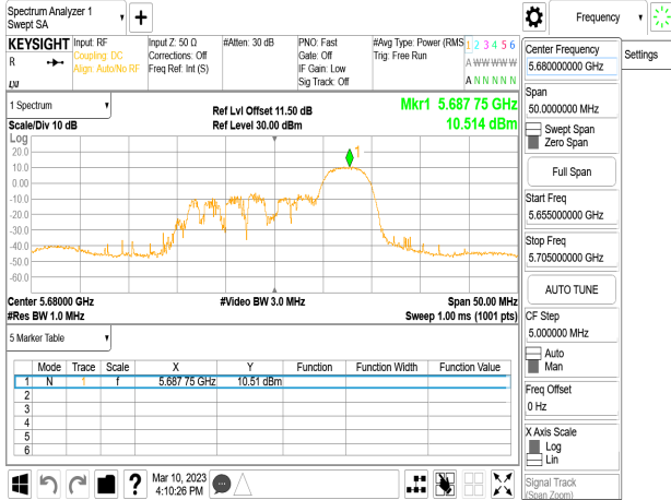
802.11ax_20MHz_Chain0_5680MHz_SU
