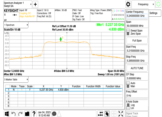
802.11ax_20MHz_Chain0_5240MHz_RU106_53
