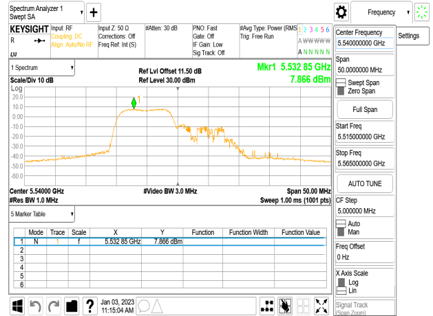
802.11ax_20MHz_Chain0_5540MHz_RU106_54
