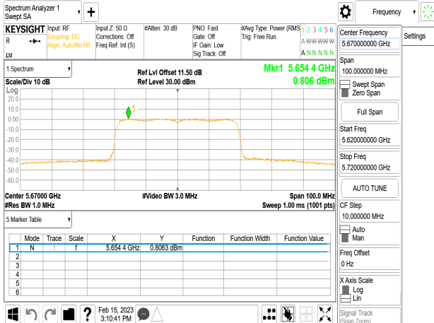
802.11ax_40MHz_Chain0_5670MHz_SU
