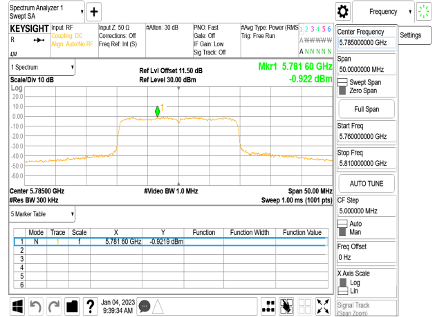
802.11ax_20MHz_Chain0_5785MHz_RU106_53
