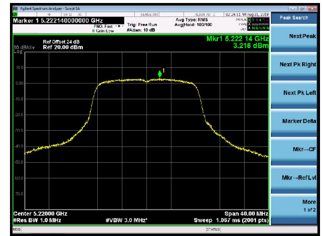
Channel 44 (5220MHz)
