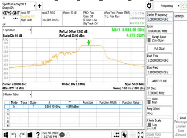
802.11ax_20MHz_Chain0_5680MHz_RU106_54
