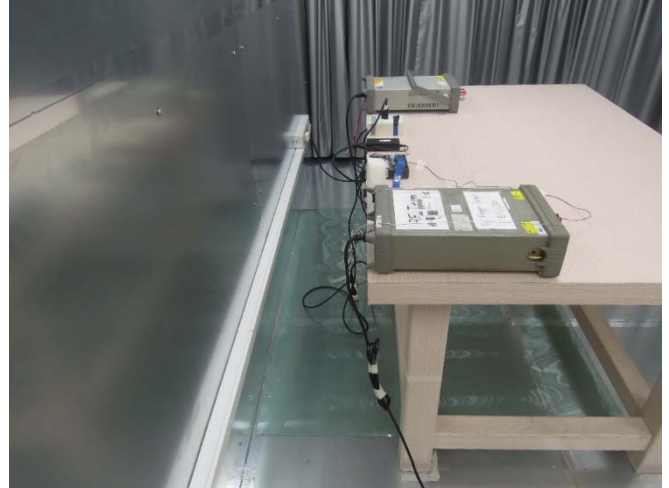
Part_15_407_WLAN_6E_Conduction_Setup
