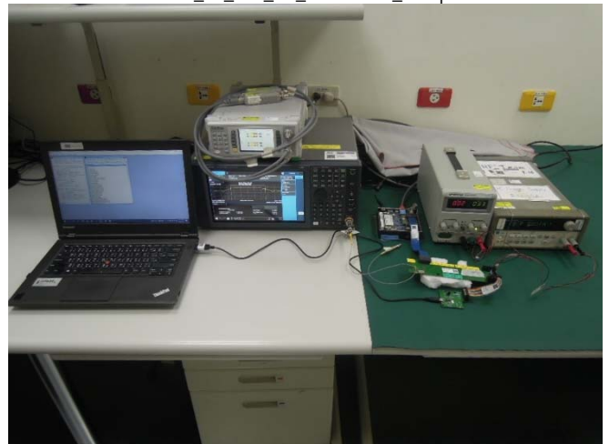
Part_15_247_LE_Conducted_Setup
