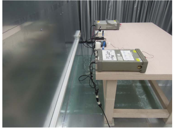
Part_15_407_WLAN_5G_Normal_DFS_Setup
