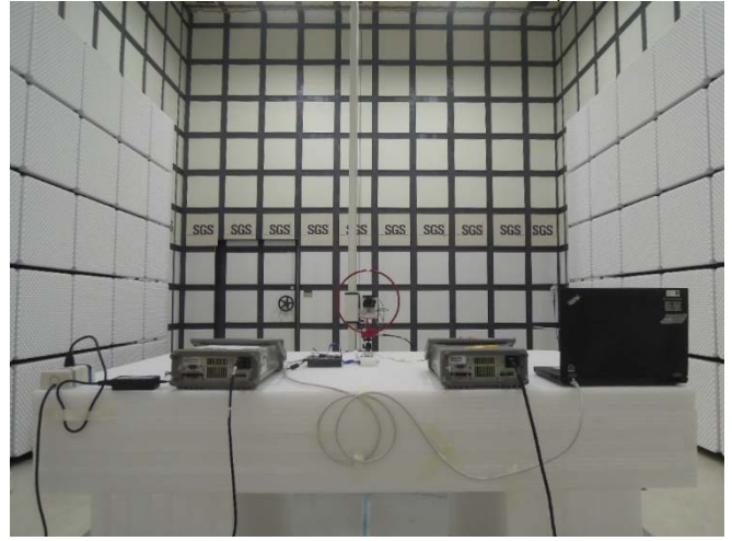
Part_15_407_WLAN_6E_Conduction_Setup
