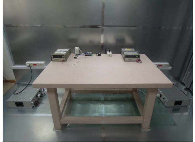
Part_15_407_WLAN_6E_Conduction_Setup
