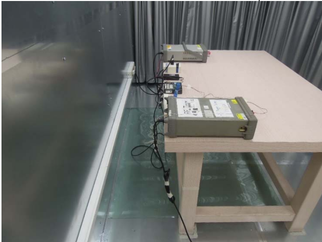
Part_15_247_WLAN_2.4G_Conducted_Setup
