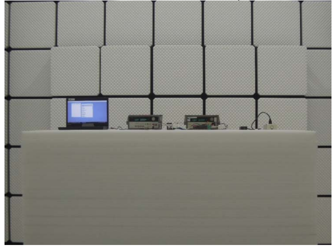
Part_15_247_BT_Radiated_Setup
