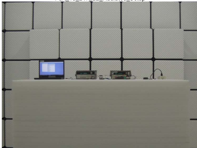
Part_15_247_LE_Radiated_Setup
