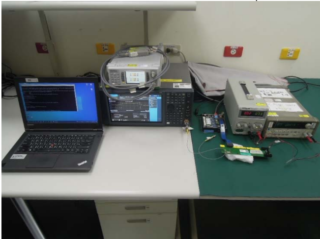
Part_15_247_WLAN_2.4G_Conducted_Setup
