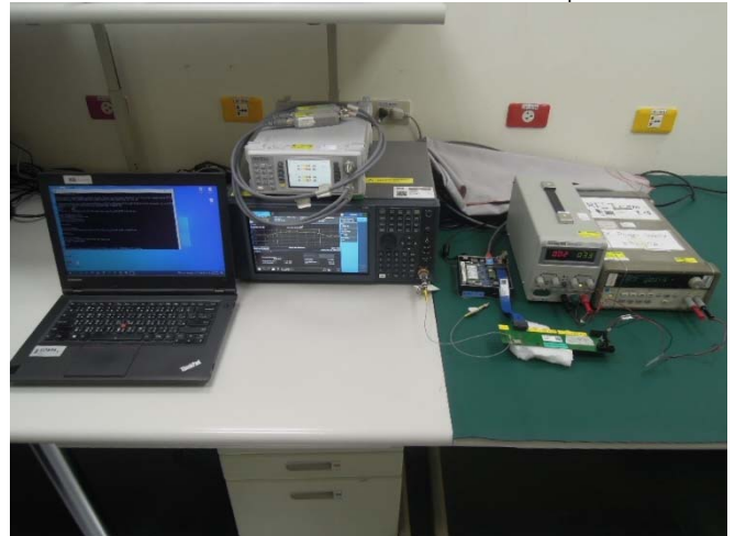
Part_15_407_WLAN_6E_Conducted_Setup
