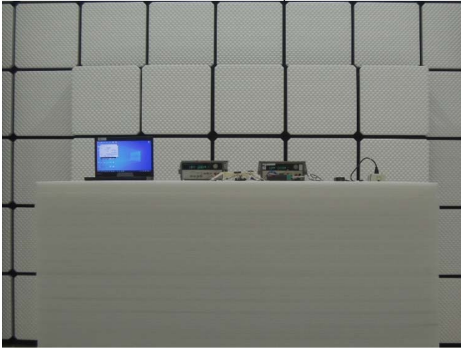
Co-location_Setup
