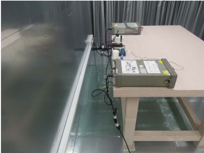
Part_15_247_WLAN_2.4G_Conduction_Setup
