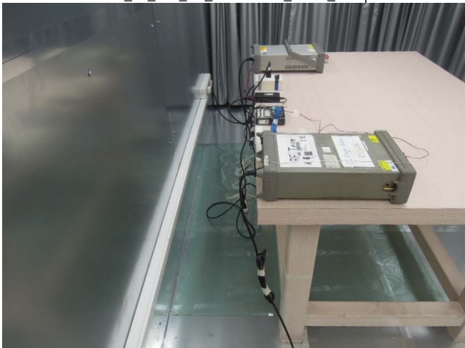
Part_15_247_BT_Conduction_ANT0_Setup
