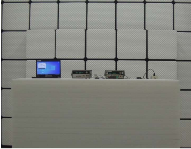
Part_15_407_WLAN_6E_Radiated_Setup
