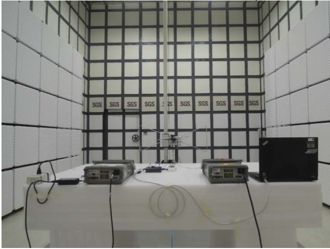
Part_15_407_WLAN_5G_Radiated_Setup
