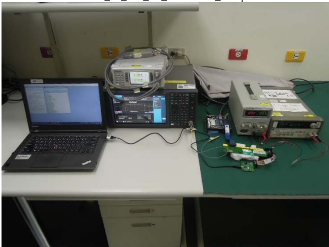
Part_15_247_BT_Conducted_Setup
