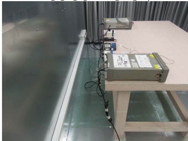
Part_15_247_LE_Conduction_ANT0_Setup
