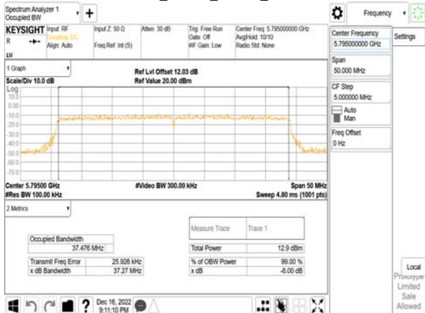
802.11ax_40MHz_Chain0_5795MHz
