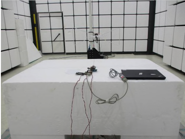
Part_15.407_WLAN_Radiated_monopole_Setup
