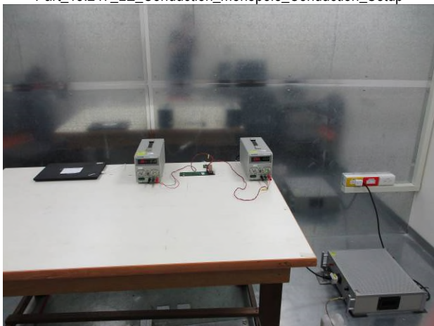
Part_15.247_LE_Conduction_monopole_Conduction_Setup
