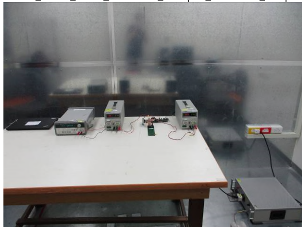
Part_15.247_WLAN_Conduction_monopole_Conduction_Setup
