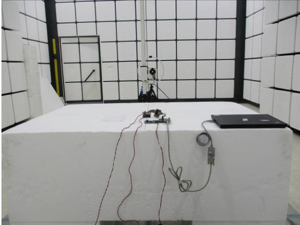
Part_15.247_BT_Radiated_dipole_Setup
