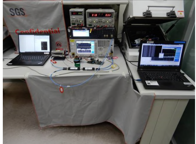
Part_15.407_WLAN_Normal_DFS_Setup
