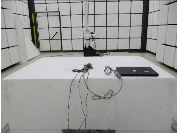
Part_15.247_WLAN_Radiated_monopole_Setup
