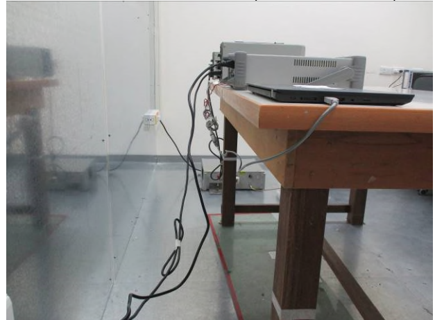
Part_15.407_WLAN_Normal_DFS_Setup
