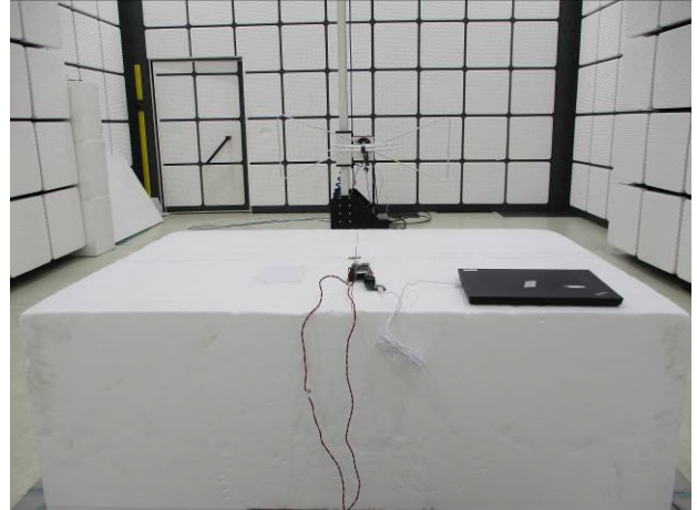
Part_15.247_BT_Radiated_dipole_Setup
