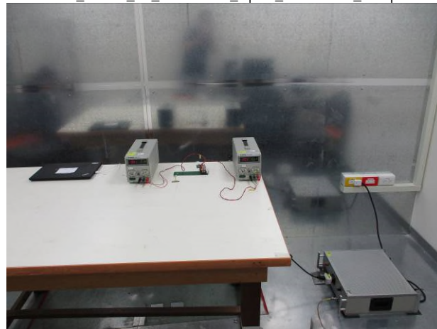
Part_15.247_LE_Conduction_dipole_Conduction_Setup
