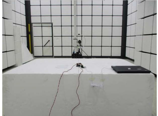
Part_15.247_LE_Radiated_monopole_Setup
