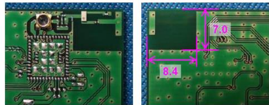
<Antenna area>
