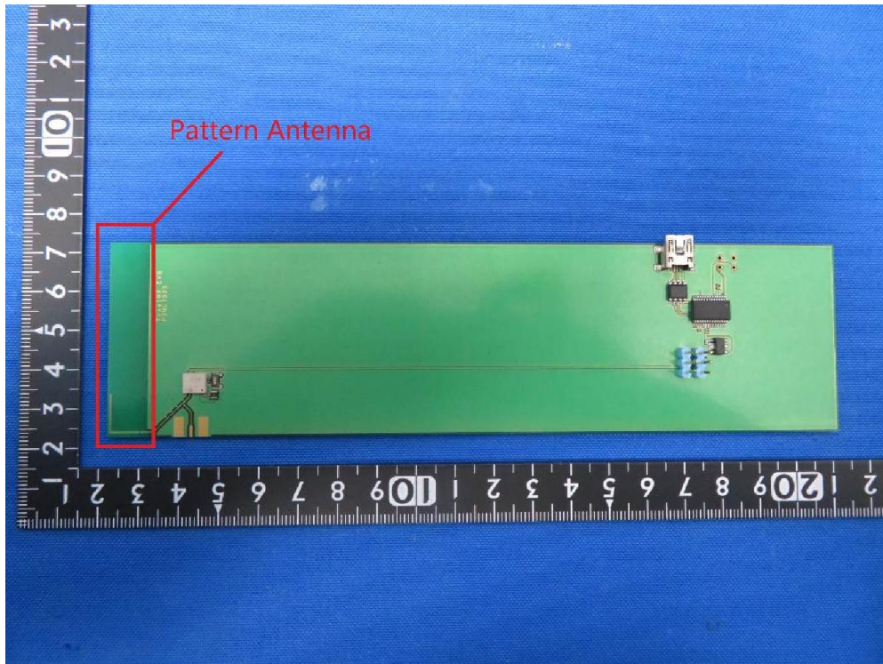
(6) EUT Photo (Test Fixture and EUT)
