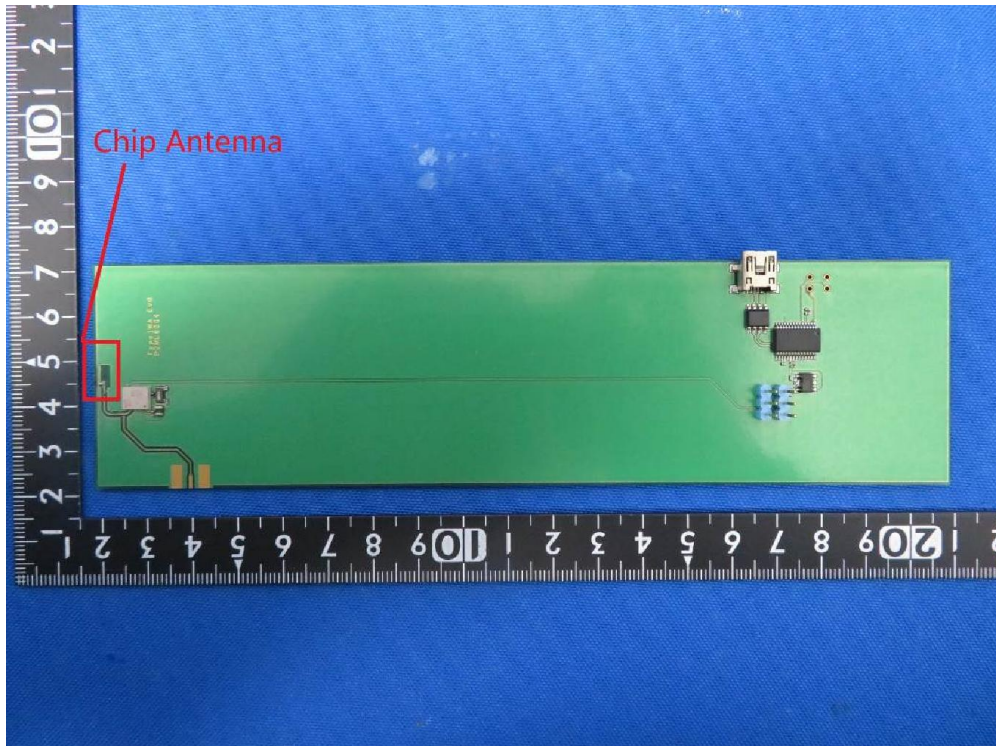
(1) EUT Photo (Test Fixture and EUT)
