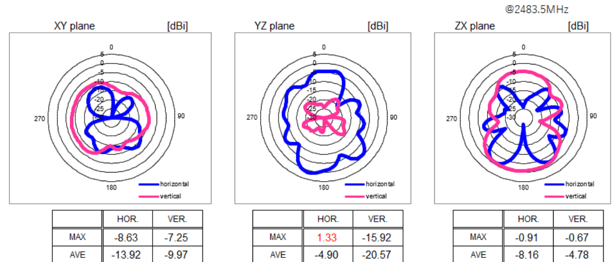
<Directivity>
