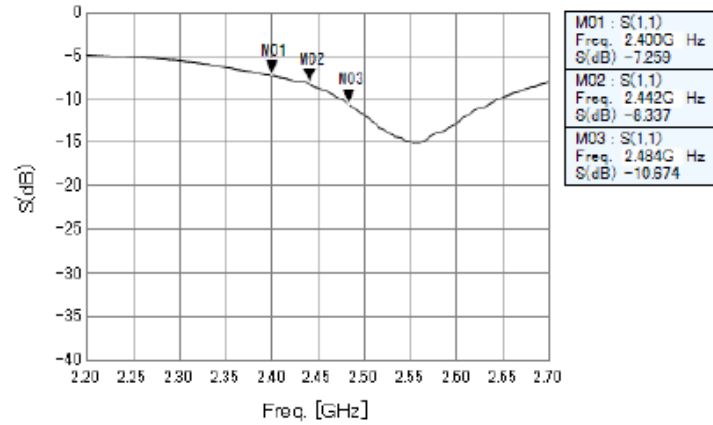
<Return Loss>
