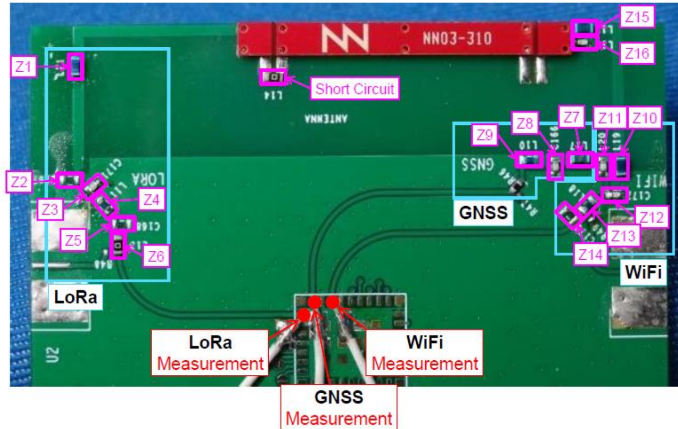
Antenna placement
