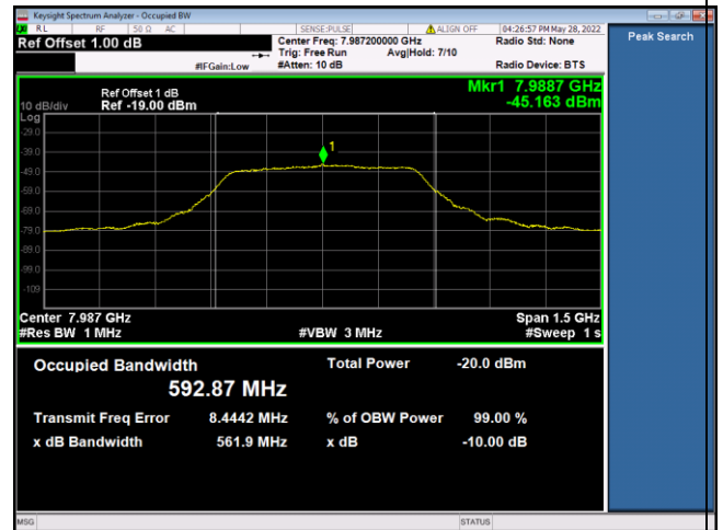
7987.2MHz_BPRF_SP 0_Payload 64
