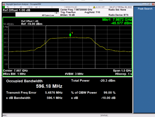
7987.2MHz_BPRF_SP 0_Payload 127
