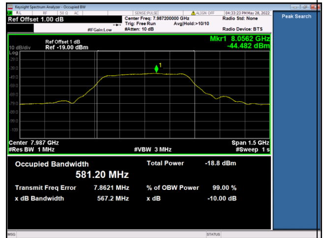
7987.2MHz_HPRF1_SP 0_Payload 512
