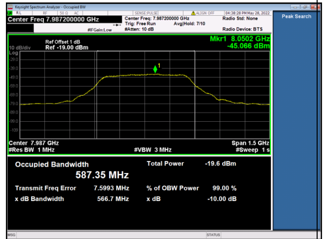
7987.2MHz_HPRF2_SP 0_Payload 512
