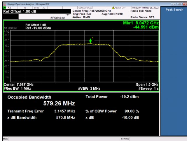
7987.2MHz_HPRF1_SP 0_Payload 2
