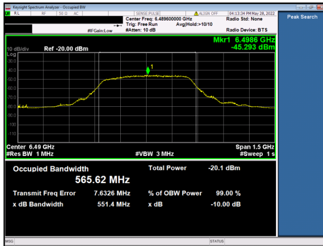
6489.6MHz_HPRF2_SP 0_Payload 2
