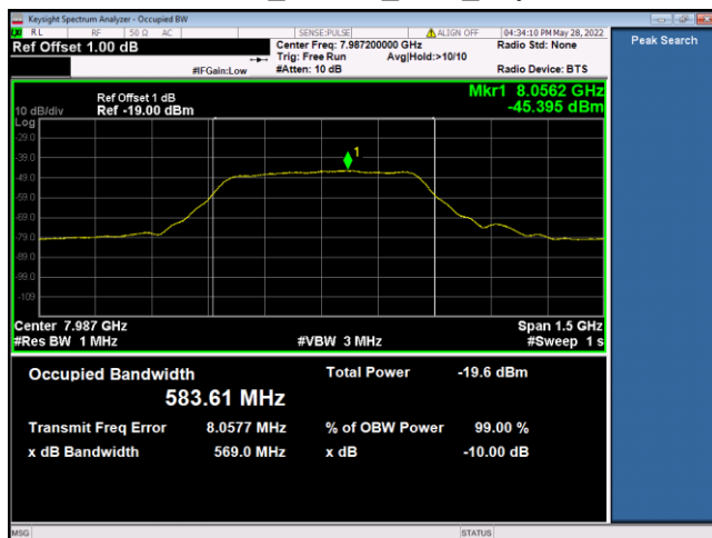
7987.2MHz_HPRF1_SP 0_Payload 1023
