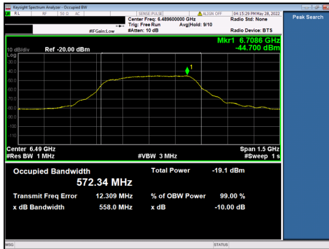
6489.6MHz_HPRF2_SP 0_Payload 1023
