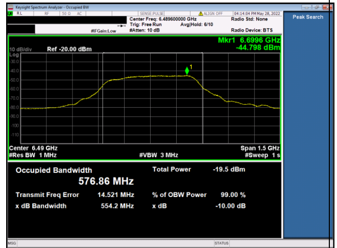
6489.6MHz_HPRF2_SP 0_Payload 512
