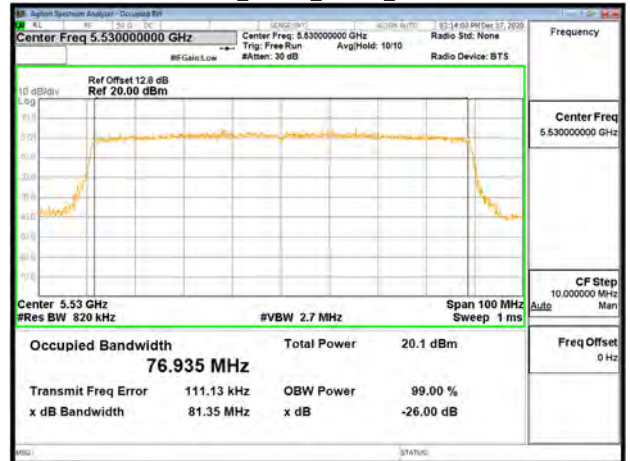
802.11ax_80MHz_Chain0_5530MHz
