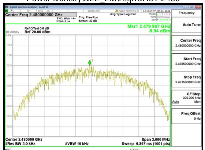
Power Density\BLE_2M\HighCH39-2480
