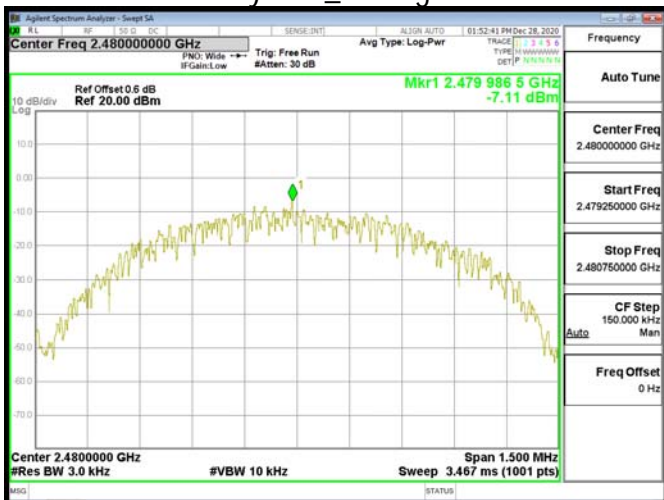
Power Density\BLE_1M\HighCH39-2480
