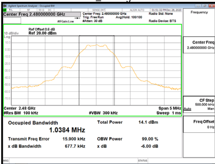
OBW 6dB\BLE_1M\HighCH39-2480
