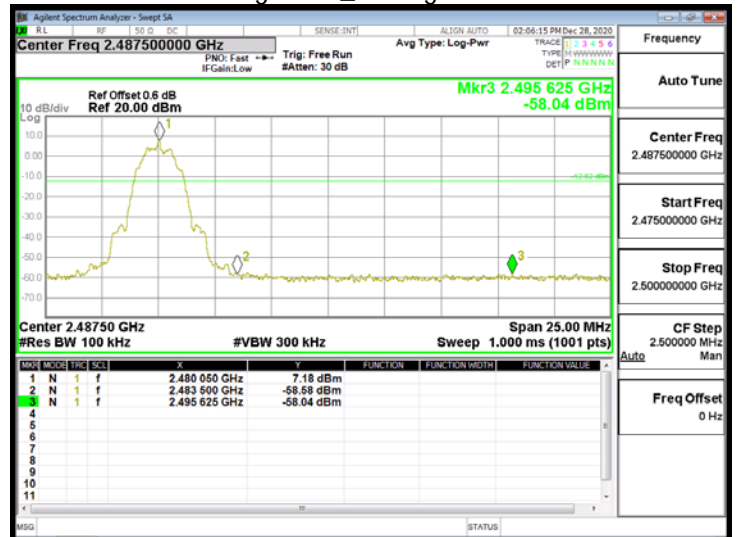
Band EdgeBLE_2MHighCH39-2480
