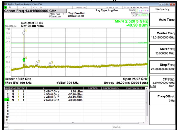
Spurious Emission\BLE_2M\HighCH39-2480
