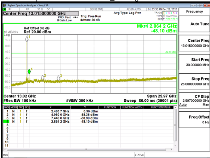
Spurious Emission\BLE_1M\HighCH39-2480
