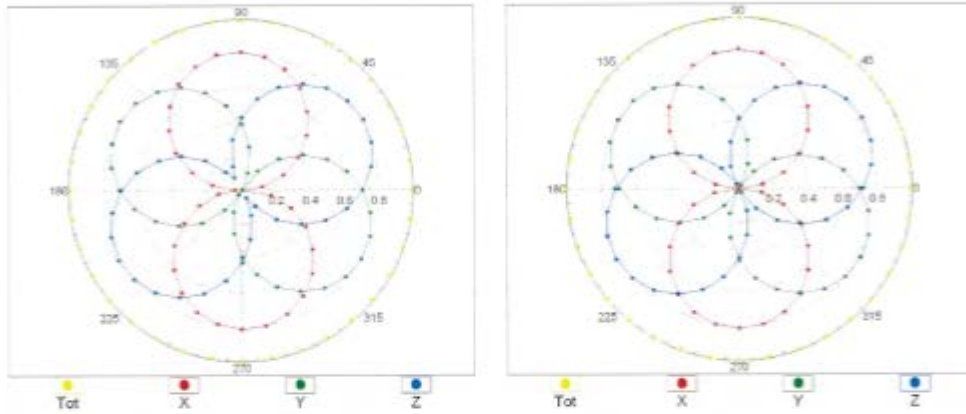
f=600 MHz,TEM
